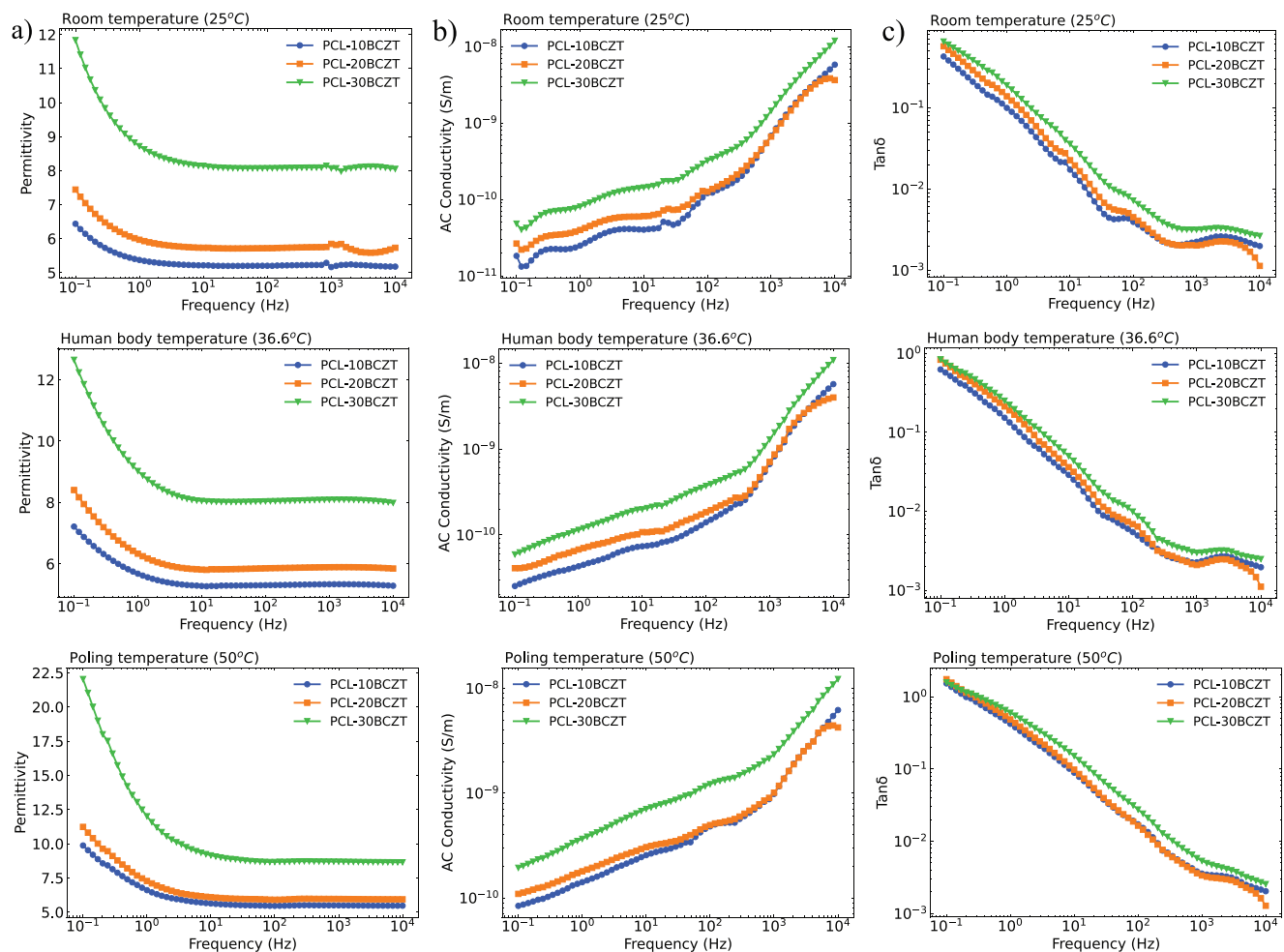
Figure 6. Dielectric response of the 3D printed ferroelectric composites as a function of frequency at three different temperatures: a) Real part of dielectric permittivity, b) AC Conductivity ( S\ m^{-1} ), and c) Loss tangent ( \tan\delta ).
