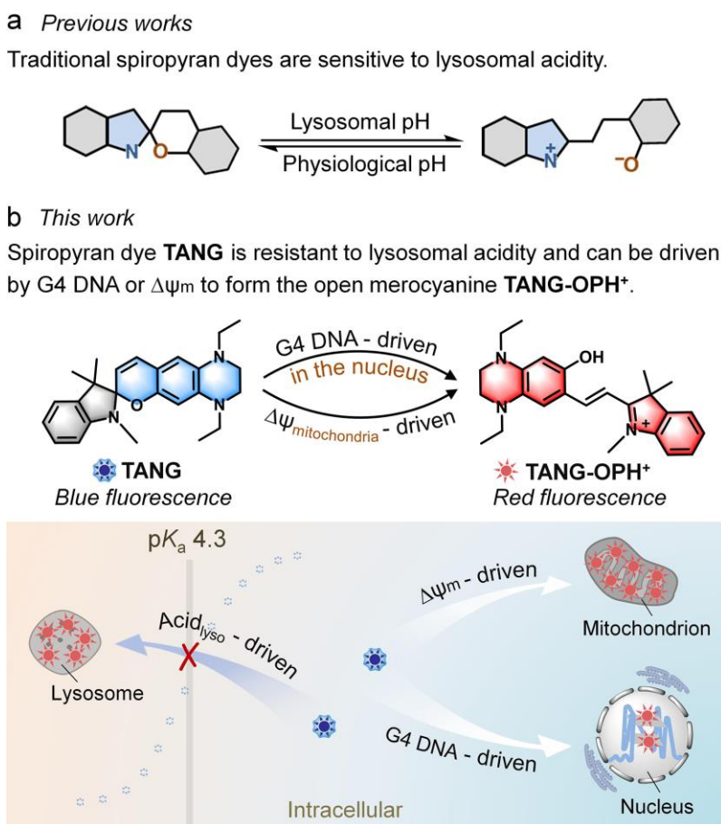
Fig. 1. (a) Illustration of traditional spiropyran dyes sensitive to lysosomal acidity. (b) Working principle of TANG with resistance to lysosomal acidity for sensing of G4 DNA or changes of \Delta\Psi_m resulting in the open merocyanine form TANG-OPH + .
