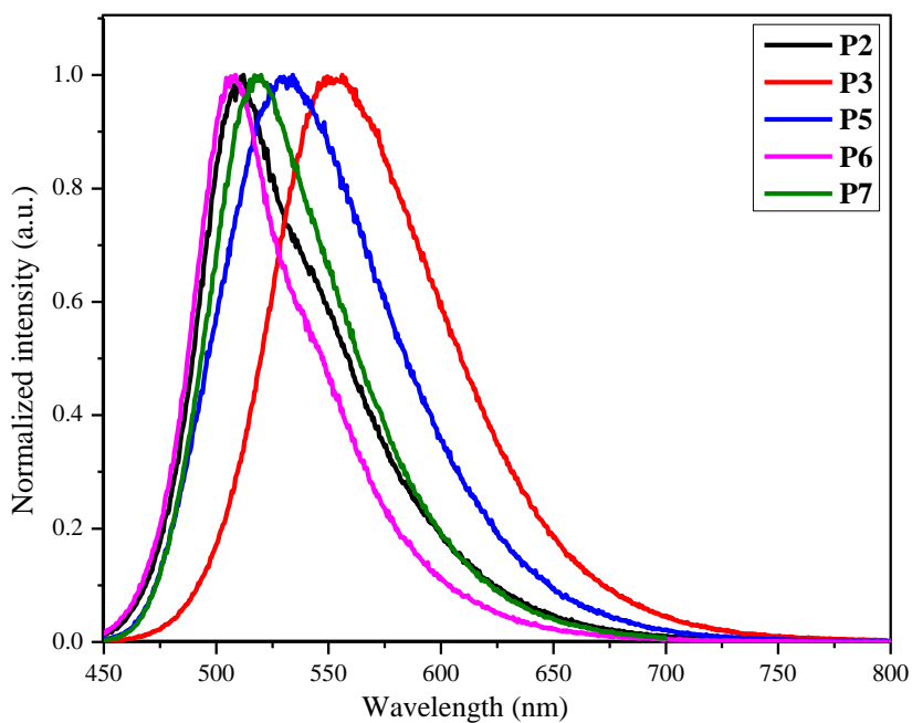
Figure 2 Room temperature fluorescence emission spectra of the organic co-poly-yne P2 , P3 , P5 – P7 in 10^{-5} M \text{CH}_2\text{Cl}_2 solution collected at the excitation wavelengths listed in Table 2 .
