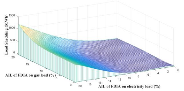
Fig. 6. Power load shedding under P-FDIA and G-FDIA.
