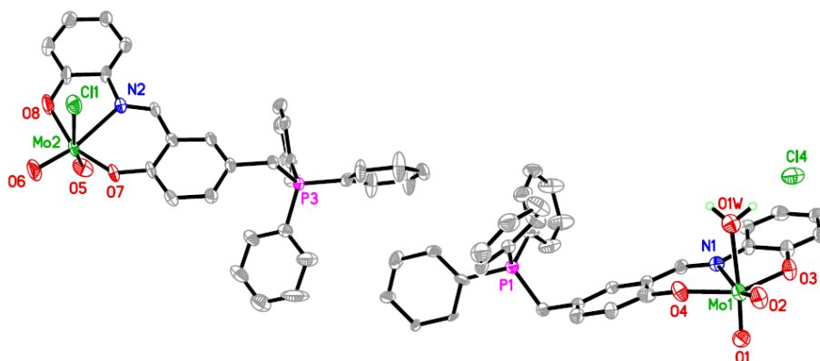
Figure 3. The ORTEP of complex 4 with selected atoms numbering and ellipsoids probability at 40%. The hydrogen atoms (except for coordinated aqua ligand) were omitted for clarity and only the major part was shown.
