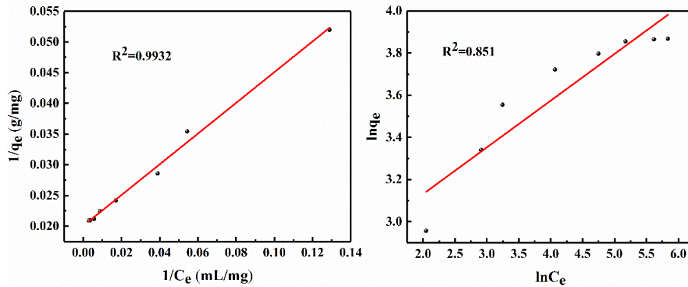
Fig. 8. Adsorption isotherms of Lyz adsorption on ZrO_2-0.02 fitted by the Langmuir (left) and Freundlich (right) models
