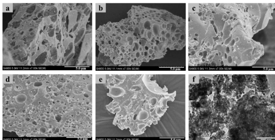
Fig. 2. SEM image of ZrO_2 synthesized using 0.01 mol P123, 0.7 mol Zr(SO_4)_2 and different content of AMTE (a~e: 0.01, 0.02, 0.03, 0.04, 0.05 mol AMTE, respectively, marked ZrO_2 -0.01, ZrO_2 -0.02, ZrO_2 -0.03, ZrO_2 -0.04, ZrO_2 -0.05, respectively) (f) TEM images of ZrO_2 -0.02
