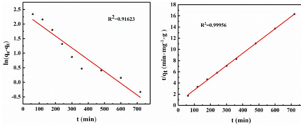
Fig. 7. Adsorption kinetic data of Lyz onto ZrO_2-0.02 fitted by two kinetic (PFO (left) and PSO (right)) equations.
