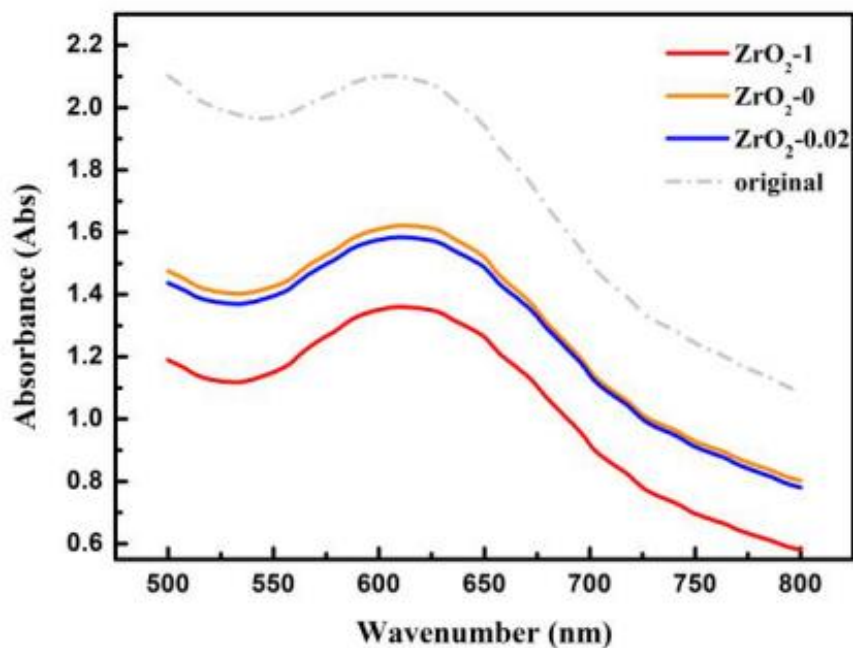
Fig. 10. UV spectrum of leather softening wastewater. The gray dashed line represents the original wastewater before adsorption. The red, orange and blue curves represent the wastewater adsorbed by ZrO 2 -1, ZrO 2 -0 and ZrO 2 -0.02, respectively. The reduction of absorbance indicates that the proteins were adsorbed by the ZrO 2 materials.
