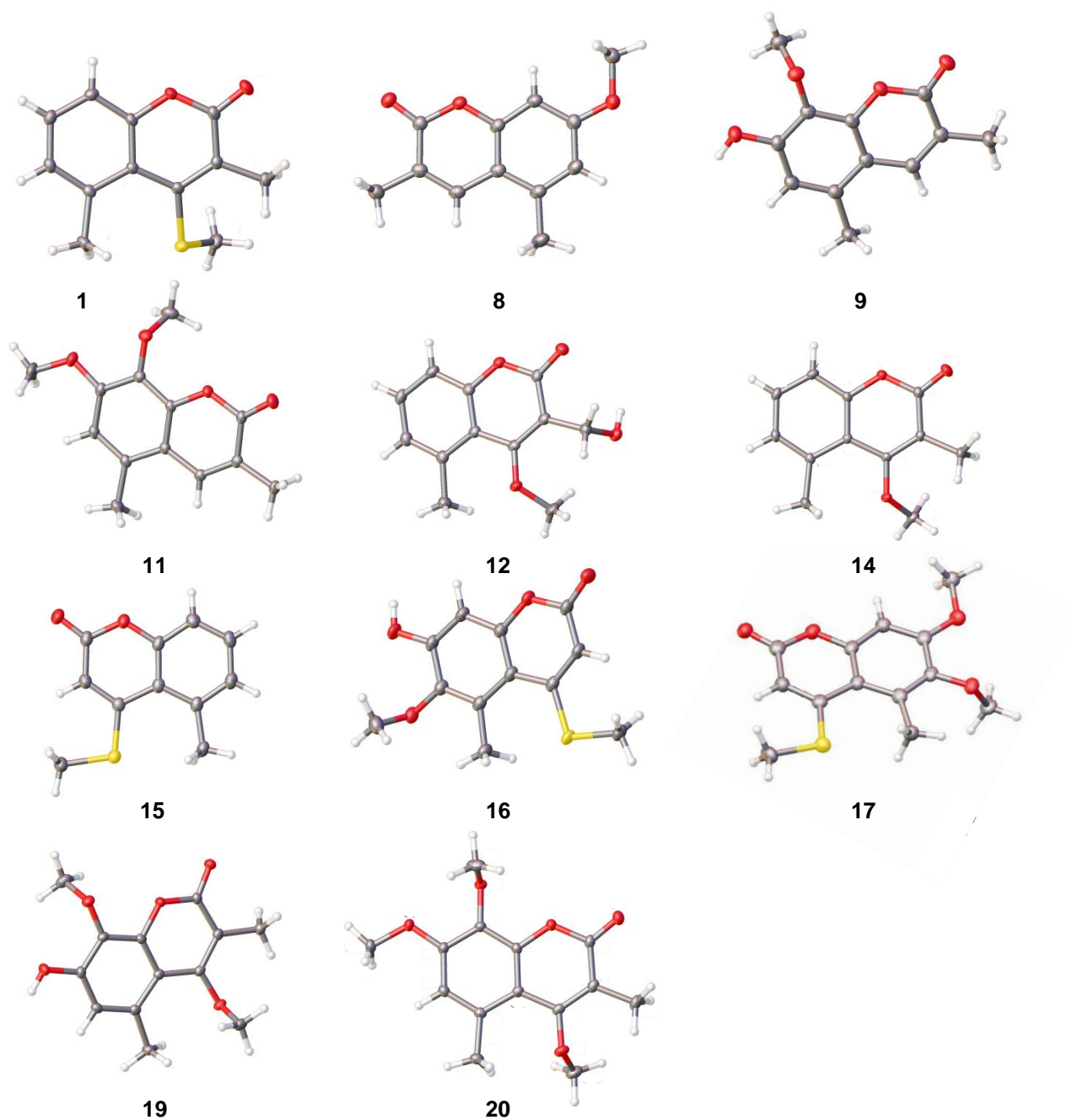
Fig. 2. X-Ray crystal structures determined for 1,8,9,11,12,14-17,19,20 . Atoms are shown as thermal ellipsoids drawn at the 50% probability level.
