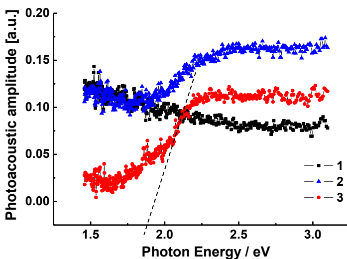
Fig.6. The photoacoustic spectra for the bare ceramic substrate (curve 1), for hematite electrode formed on the ceramic substrate (curve 2) and for hematite electrode grown on the ITO substrate (curve 3).
