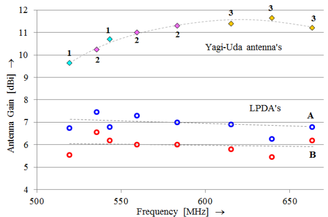
Fig. 6. Absolute antenna gain values measured with Distance Scan and calculated using the Three Antenna Method. Values can also be found in Table IV.
