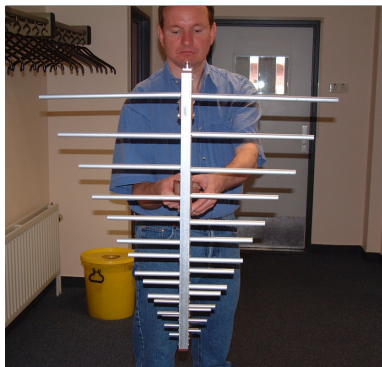
Fig. 2. The 200 MHz to 1 GHz Log-Periodic Dipole Antenna.
