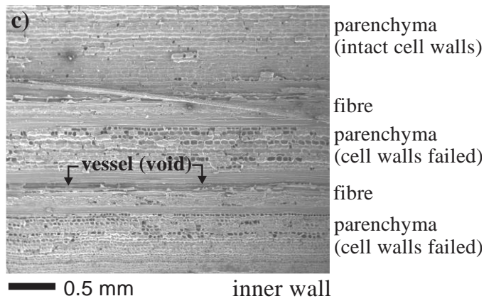
Figure 9 Detail of culm wall images of P. edulis specimen (note that images in parts b and c are not the same specimen as shown in a)
