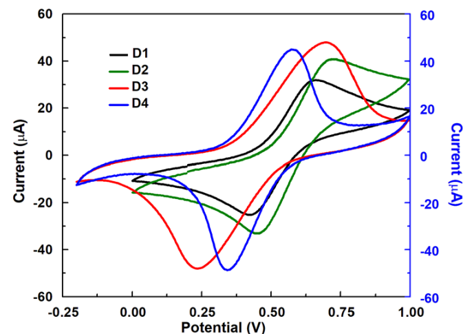
Fig 6 Cyclic voltammogram for the dyes recorded in 10 -3 M dichloromethane solution
