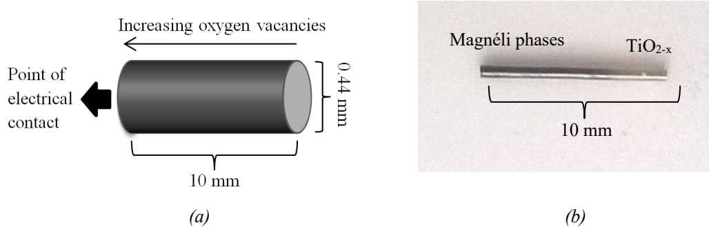
Fig. 1: (a) Schematic representation of the composite structure of a single fibre showing the gradient oxygen vacancies across the length of the fibre and (b) image of a functionally graded fibre
