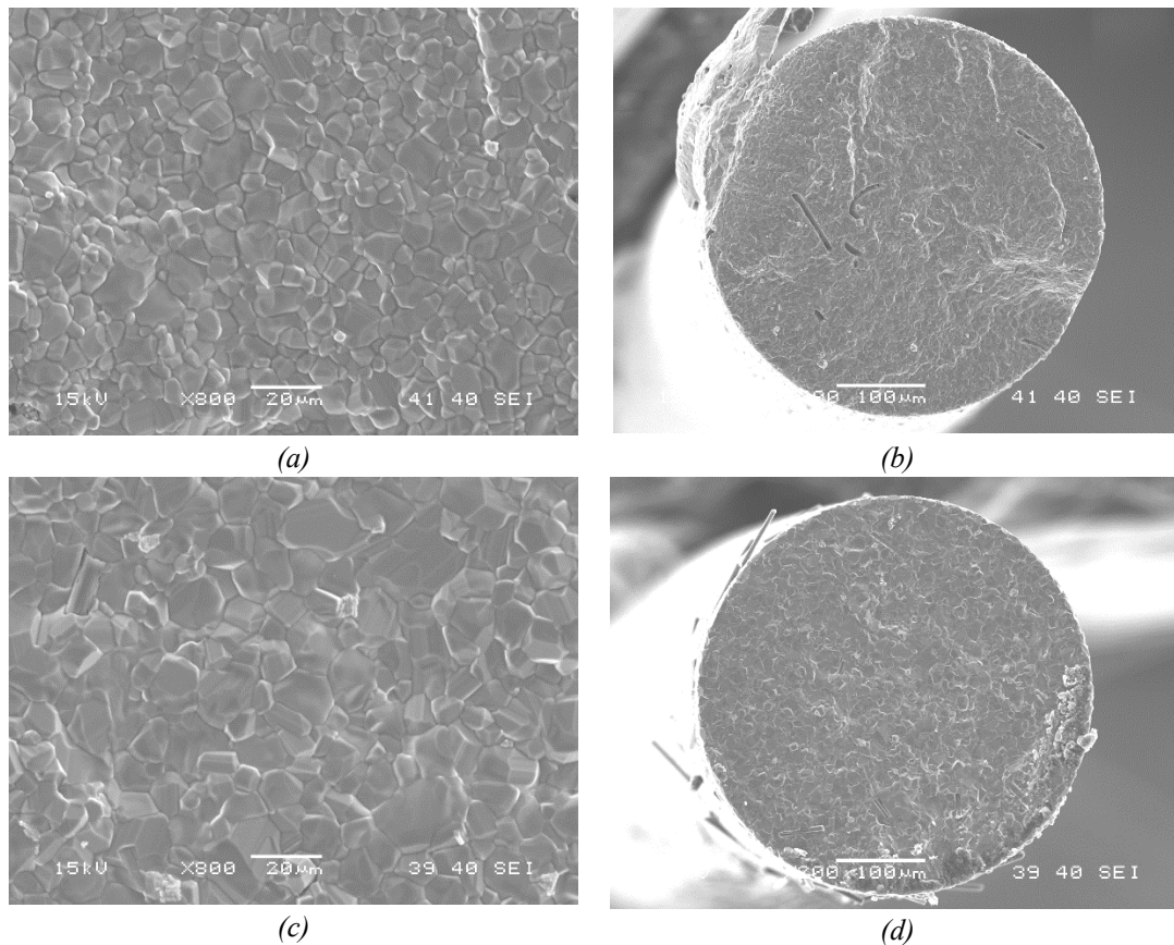
Figure 2: SEM images of (a-b) the TiO_{2-x} end of functionally graded fibres and (c-d) the Magnéli phases end of the functionally graded fibres.
