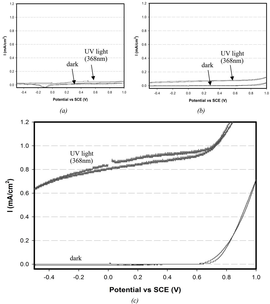
Figure 5: Photocurrent vs potential (vs SCE) under UV light of (a) \text{TiO}_2 fibre, (b) Magnéli phases fibre and (c) functionally graded fibre (760 \text{W/m}^2 , 368nm).
