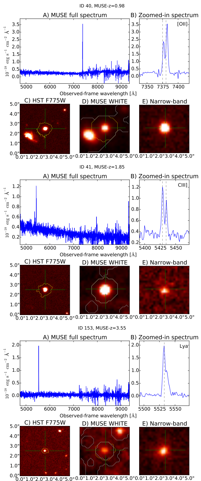
Fig. 5. Full MUSE spectrum and a zoomed-in portion of the [O II], C III], and Ly \alpha detected wavelength region at the top of each panel, and the HST F775W, MUSE white-light, and narrowband images of each emission line in the bottom of each panel. The yellow contours in the images are the boundary of the UVUDF catalog segmentation for the object, but those in the MUSE white-light image are convolved with the MUSE beam size. The white boundaries indicate masked objects excluded from local sky residual estimates. The green cross indicates the central position of the extracted object. The ID numbers and measured redshift are indicated at the top of each panel. All of these redshifts are secure (CONFID = 2 or 3).
