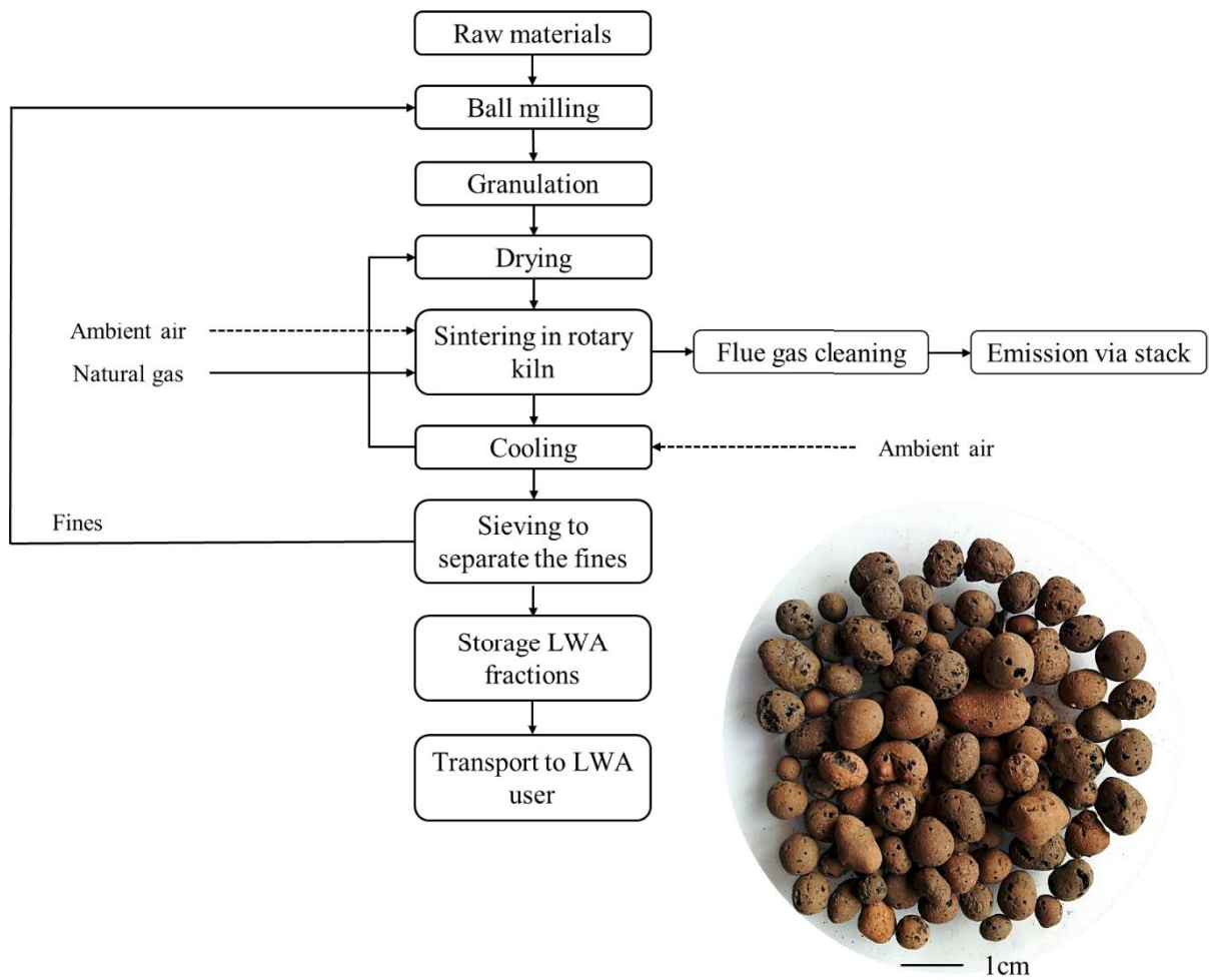
Fig. 1. Lightweight aggregate (LWA) manufacturing process flowchart and typical clay LWA end product [1].
