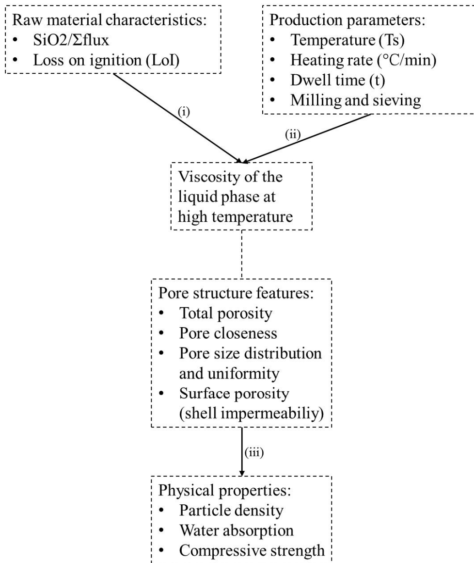
Fig. 2. Relationships between raw material characteristics, production parameters and mechanical properties, showing the pore structure as an intermediate variable.
