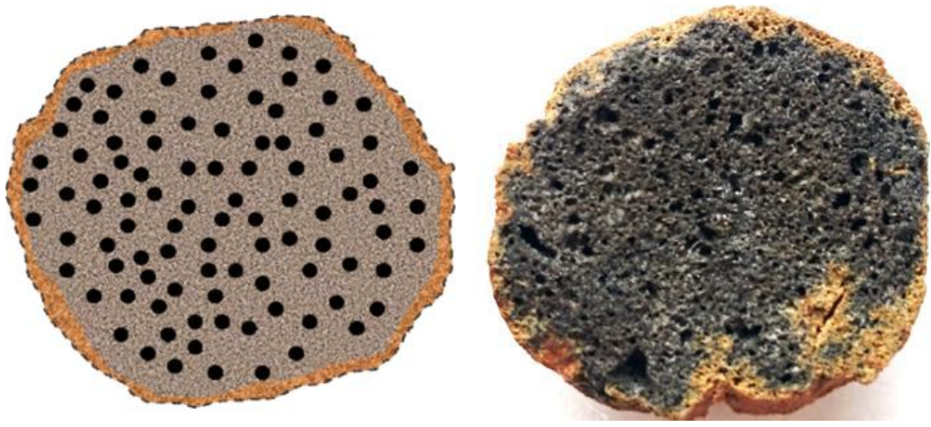
Fig. 3. Schematic of an ideal pore structure (left) and typical pore structure of clay LWA (right).
