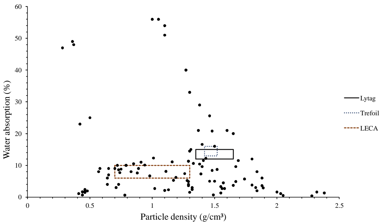
Fig. 5. Relationship between particle density and water absorption of the reviewed manufactured LWAs. Lytag: straight black line, Lightweight expanded clay aggregate (LECA): brown dashed line, Trefoil: blue dashed line.
