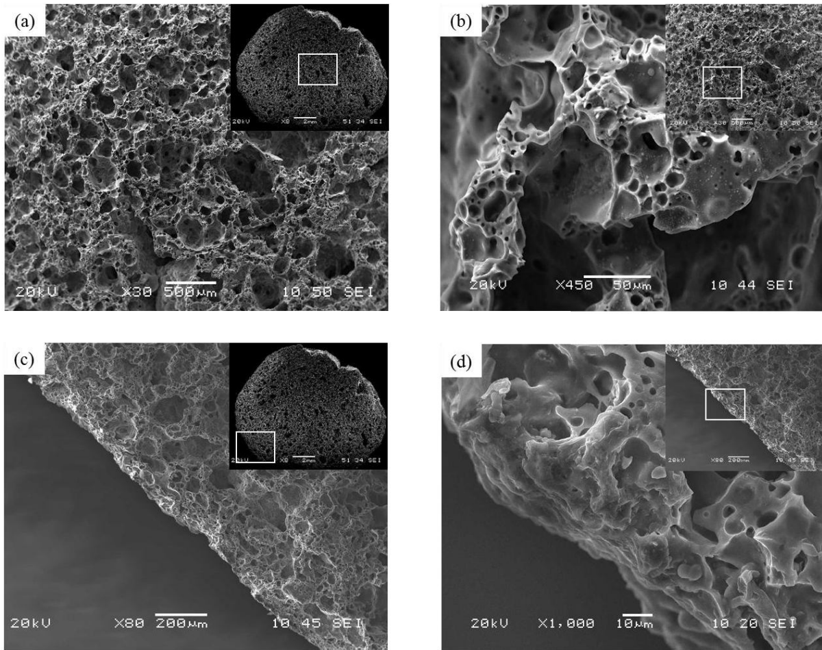
Fig. 4. SEM micrographs of fracture surface of a clay LWA granule, taken from Sustainability Research Institute SEM archive (unpublished data): (a) LWA core pore structure, (b) core at a higher magnification, (c) LWA shell cross-section and, (d) shell cross section at a higher magnification.
