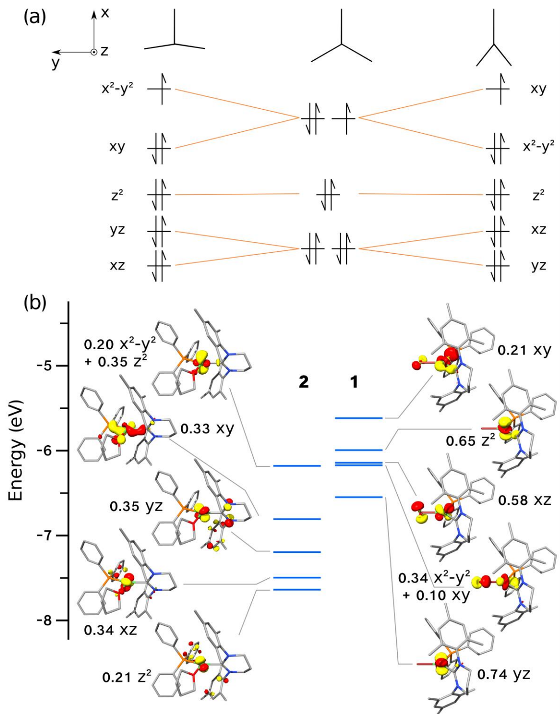
Fig. 10. (a) Schematic molecular orbitals diagrams expected for three-coordinate d^9 complexes, left to right: T-shaped, ideal D_{3h} , Y-shape; a larger ligand field splitting
