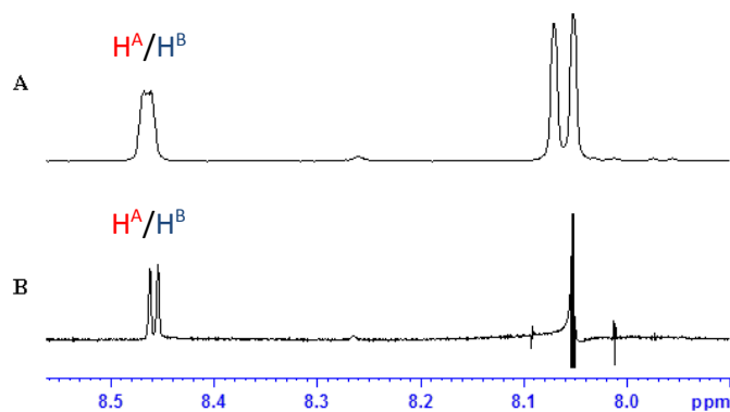
Figure 2 - Expansion of the aryl region of the 500 MHz ^1\text{H} NMR spectrum of the 50:50 mixture of homochiral:heterochiral diastereomers formed from reaction of racemic dibenzyl-DL-tartrate with 1,3-phenyldiboronic acid. (A) Poor resolution observed for \text{H}^{\text{A}}/\text{H}^{\text{B}} resonances using standard ^1\text{H} NMR processing techniques; (B) Baseline resolution observed for \text{H}^{\text{A}}/\text{H}^{\text{B}} resonances using Gaussian enhancement of a ^1\text{H}\{^1\text{H}\} decoupling experiment.
