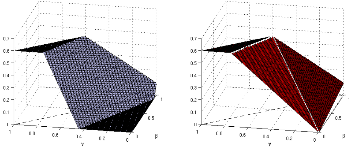
FIGURE 1. The modified cost function \bar{f}(\beta, \gamma) on the left plotted together with the projected value function V_\alpha(\beta, \gamma) on the right for K_1 = -0.1 and K_2 = 0.5 . The three triangular planar regions correspond to the three cases above. It is evident that V_\alpha(\beta, \gamma) is the concave envelope of \bar{f}(\beta, \gamma) .
