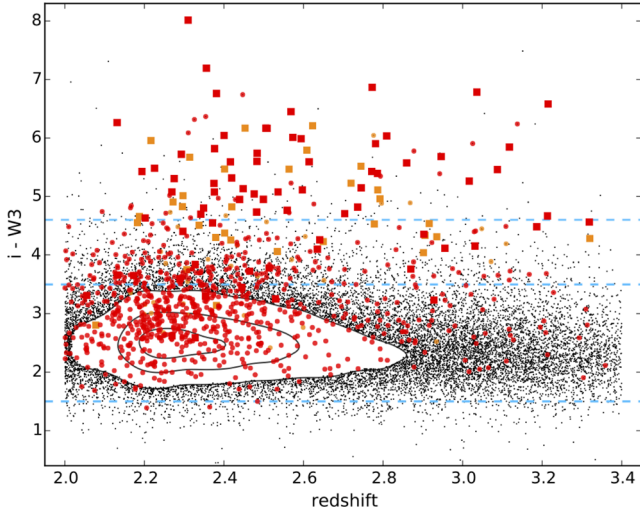
Figure 9. i-W3 colour versus redshift for the W3-detected sample. The red/orange symbols mark type 1/2 quasars with \text{REW}(\text{C IV}) \geq 100 \text{ \AA} , while the squares identify subsets of these quasars with wingless profiles, e.g. kt_{80} > 0.33 . The dashed blue lines mark specific colours i - W3 = 1.5, 3.5 and 4.6 used to construct composites for Fig. 11 below (Section 4.5).
