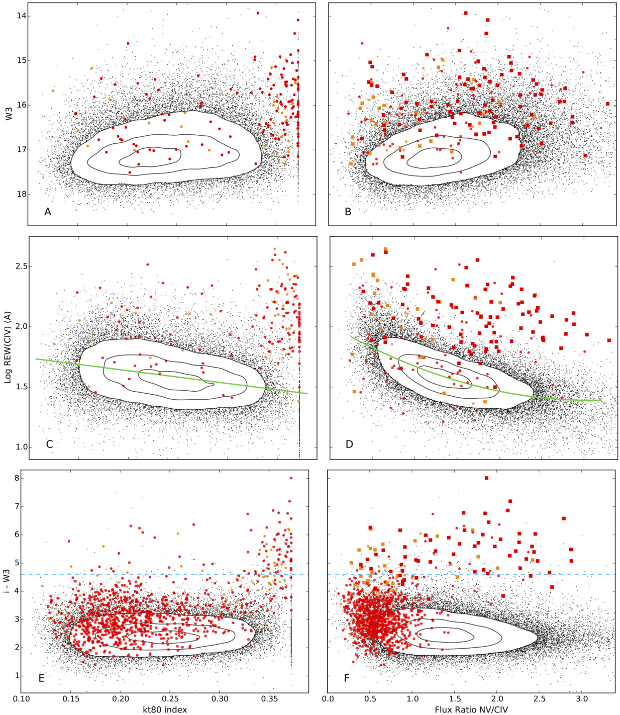
Figure 7. Kurtosis index kt_{80} for C IV (left-hand panels) and line flux ratio N_V/C_{IV} (right-hand panels) versus W3 magnitude (top), \log \text{REW}(C_{IV}) in Å (middle), and i-W3 colour (bottom) for quasars in the W3 -detected sample. In the top two rows (panels A-D), the red and orange symbols mark Type 1 and 2 ERQs, respectively defined by i-W3 \geq 4.6 . In the bottom row (panels E-F), the red and orange symbols mark all Type 1 and 2 quasars, respectively, with \text{REW}(C_{IV}) \geq 100 Å. The dashed blue line marks the ERQ threshold at i-W3 = 4.6 . In the right-hand panels, the square red and orange symbols additionally indicate kt_{80} > 0.33 . Quasars with weak lines bunched up at kt_{80} = 0.37 are artefacts of the fitting procedure, which defaults to a single Gaussian if the fit is not improved by a second component. The green curves in panels C and D are fits to the point distributions intended only to guide the eye.
