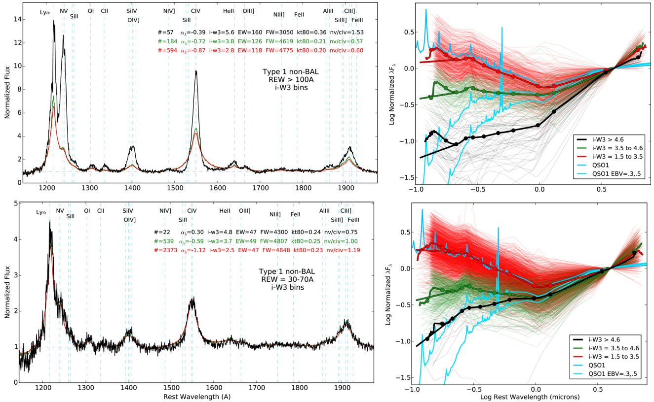
Figure 11. Top row: normalized median BOSS spectra (left) and SEDs (right) for Type 1 non-BAL W3 -detected quasars with \text{REW}(C\text{IV}) \geq 100 \text{ \AA} in the three colour bins shown in Fig. 9: ERQs with i-W3 \geq 4.6 (black curves), intermediate colours 4.6 > i-W3 \geq 3.5 (green curves), and blue quasars with 3.5 > i-W3 > 1.5 (red curves). The left-hand panels provide median values of some measured parameters for these quasar samples, as in Fig. 8 above. The SEDs are scaled to unity at 4 \mu\text{m} and plotted with the same colour scheme as the BOSS spectra. The thin faint curves are individual quasar SEDs while the bold curves are the sample medians. The dots on the bold median SEDs mark wavelengths of the broad-band filters at a typical redshift z_e = 2.5 , from left to right: griz , YJHK , and W1 , W2 , W3 and W4 . The median SEDs split at short wavelengths to show results directly from the photometry (upper curves with filter dots) and for a median power law derived from fits to the UV spectra of individual quasars that are more reliable because they avoid spectral line contamination (lower curves without dots). The slopes of these median UV power laws are listed in the left-hand panels. The light blue SEDs show the Type 1 quasar template QSO1 from Polletta et al. (2007) without and with reddening for E(B - V) = 0.3 and 0.5 using an SMC-like reddening curve (from Hamann et al. in preparation). Bottom row: same as above but for quasars with 30 < \text{REW}(C\text{IV}) < 70 \text{ \AA} . See Section 4.5.
