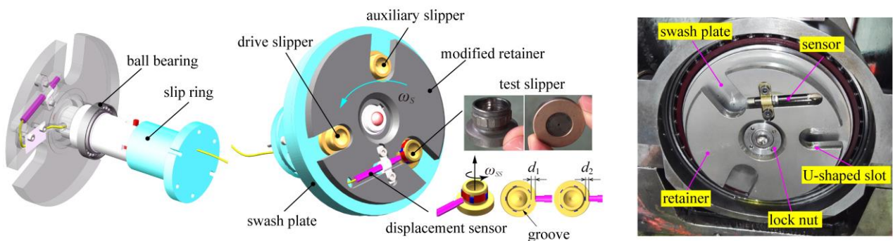
Fig. 15. Slipper spin measurement using an displacement sensor
