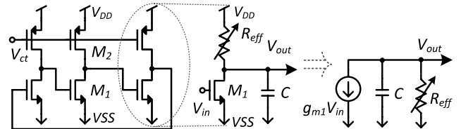
Fig. 1. Common source amplifier based RO-VCO.
