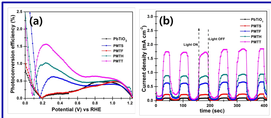
Fig. 6. (a) Photoconversion efficiency curves of structurally tuned PMT photoelectrodes under 1 sun power ( 100\text{mW cm}^{-2} ) solar simulator with a scan rate of 20\text{ mV/sec} in 0.1\text{ M Na}_2\text{SO}_4 and (b) Time dependent photo-response in PMT photoelectrodes including pristine \text{PbTiO}_3 perovskite at fixed potential of 1.23\text{ V Vs RHE} . The mass loading of the samples were \sim 2.59, 2.62, 2.63, 2.61 and 2.63\text{ mg} of \text{PbTiO}_3, \text{PMTS}, \text{PMTF}, \text{PMTH} and \text{PMTT} respectively on Nickel foam.
