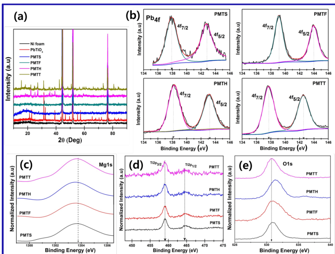
Fig. 4. (a) XRD patterns of pure Ni foam, pure PbTiO_3 and structurally tuned PMT perovskites. (b) XPS spectra of Pb_{4f} , (c) Mg_{1s} , (d) Ti_{2p} and (e) O_{1s} core-levels of structurally tuned PMT perovskites.
