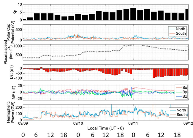
Figure 1. Geomagnetic index ( Kp ), AMIE polar cap potential, disturbance storm time index ( Dst ), Advanced Composition Explorer plasma speed and IMF strength, AMIE hemispheric power from 9 to 12 September 2005.
