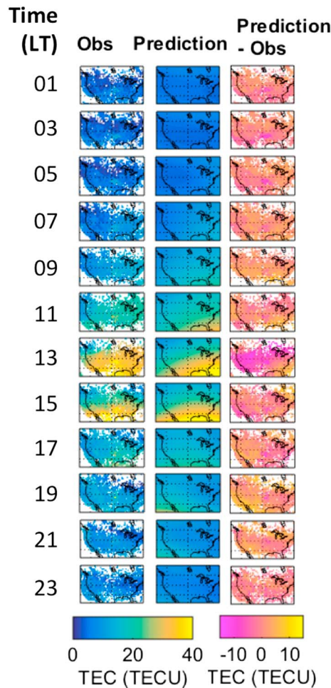
Figure 7. TEC observations, 1 h ensemble mean predictions from run (c) and the differences between the two (prediction-observations) on 10 September 2005.
