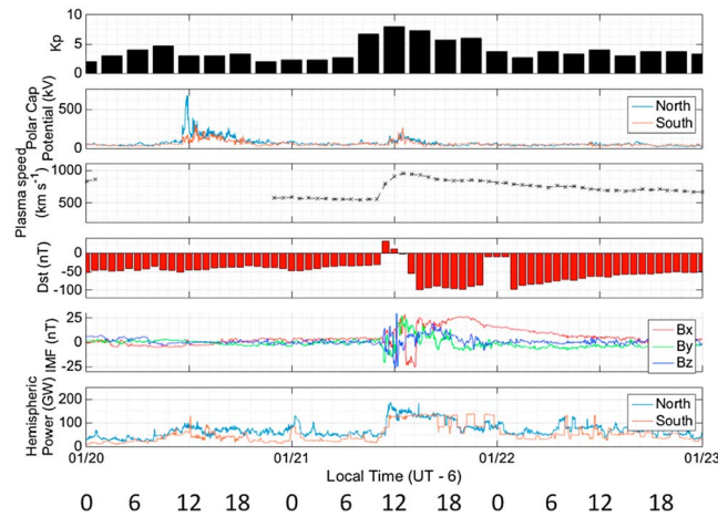
Figure 2. Geomagnetic index ( Kp ), AMIE polar cap potential, disturbance storm time index ( Dst ), Advanced Composition Explorer plasma speed, and IMF strength, AMIE hemispheric power from 20 to 23 January 2005.
