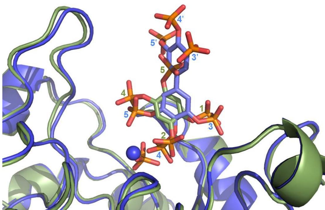
Figure 4 Overlay of Bz(1,2,4,5)P 4 -INPP5B (green) and BiPh(3,3',4,4',5,5')P 6 -INPP5B (blue) complex structures showing good overlay between the two molecules and different phosphate groups. The Mg 2+ (blue sphere) and inorganic phosphate (sticks) from the BiPh(3,3',4,4',5,5')P 6 -INPP5B structure are shown, and the numbering of the ligand phosphates are included.
