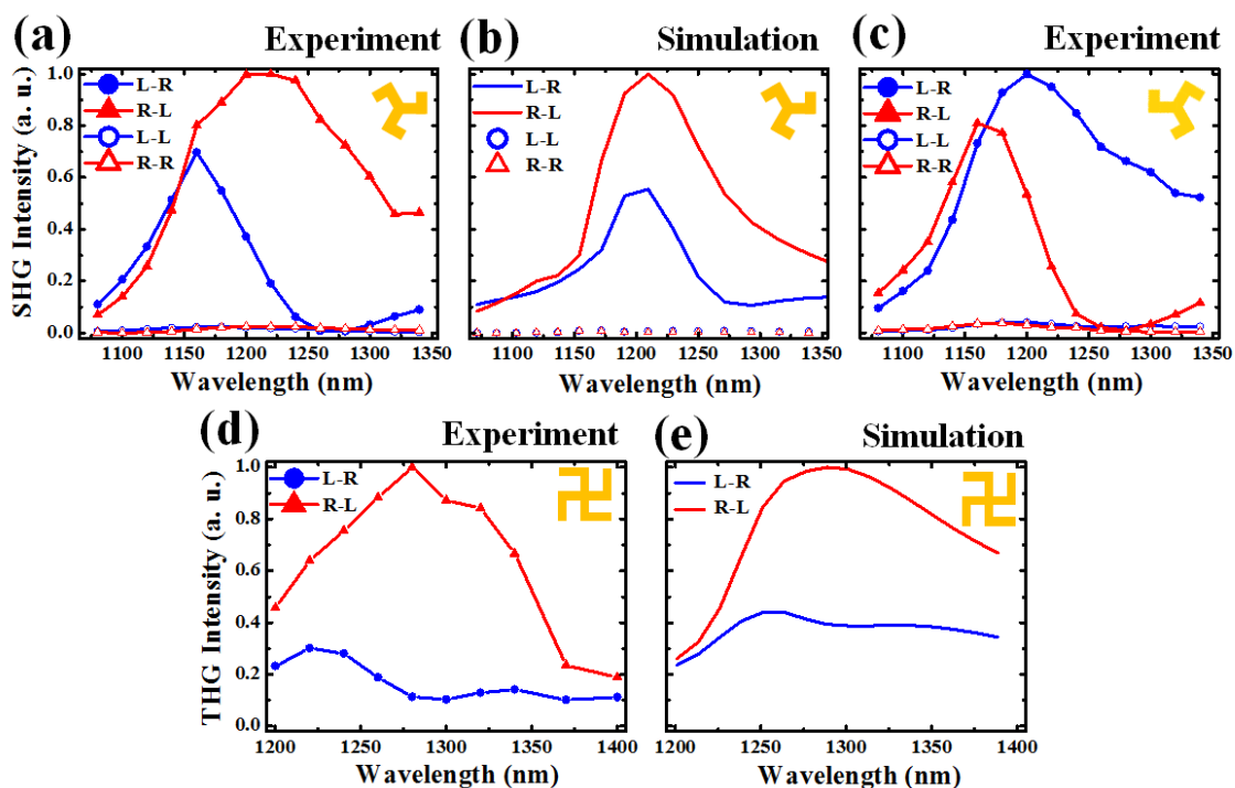
Figure 3. Polarization dependent SHG and THG spectra of the Trisceli- and Gammadion- type plasmonic nanostructures. Measured SHG and THG spectra with same (LCP-LCP and RCP-RCP) and opposite circular polarizations (LCP-RCP and RCP-LCP) as that of the illuminating light. Note, in the figure we used the abbreviation of L for LCP and R for RCP, respectively. (a, b) Measured (a) and numerically simulated (b) SHG spectra for fundamental wave normally incident from Trisceli-type nanostructure direction to substrate direction (front illumination). It is found that SHG for R-L and L-R measurements exhibit significant difference when fundamental wavelength is greater than 1160 nm, whereas L-L is close to R-R. (c) Measured SHG spectra for light incident from the substrate side (back illumination), which are very close to the results of front illumination but swapped between R-L and L-R. (d, e) Measured (d) and simulated (e) THG spectra under front illumination show pronounced difference between R-L and L-R for fundamental wavelength with a bandwidth of around 150 nm.
