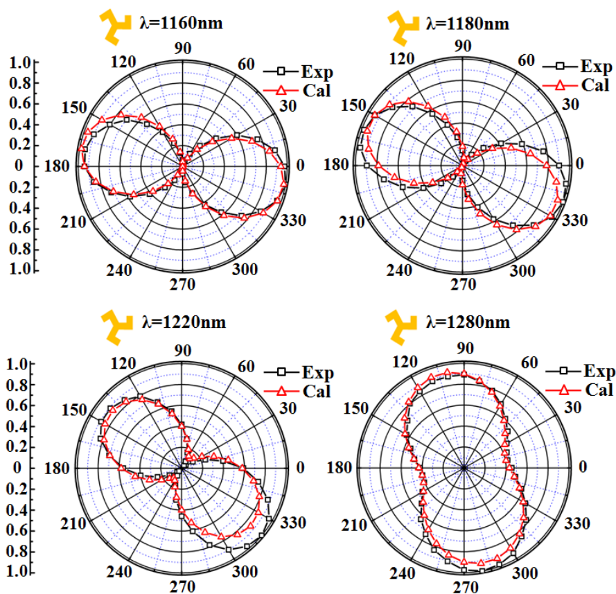
Figure 5. Intensity of the SHG signal as function of the rotation angle of the analyzer for Trisceli-type plasmonic nanostructures . The results are obtained for linearly vertically polarized (V-polarization as shown in Figure 2) illumination at wavelengths of 1160 nm, 1180 nm, 1220 nm and 1280 nm, respectively. The square and triangular symbols represent the measured (Exp) and calculated (Calc) results. By fitting the measured results, we then experimentally determine the second-order effective susceptibilities of SHG from the Trisceli-type nanostructures.
