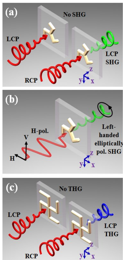
Figure 1. Schematic of nonlinear optical dichroism from Trisceli- and Gammadion- type plasmonic nanostructures with three- (C3) and four-fold (C4) rotational symmetries. (a) and (c) illustrate the nonlinear circular dichroism for illumination with LCP and RCP polarizations on such structures which will lead to SHG and THG with opposite polarizations but only for the RCP illumination. (b) Trisceli-type nanostructures with near unity SHG-CD would generate left-handed elliptically polarized SHG light when illuminated by linear polarized light.
