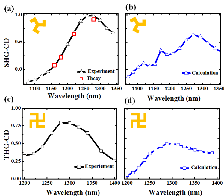
Figure 4. SHG-CD and THG-CD from the Trisceli- and Gammadion- type plasmonic nanostructures. (a) and (c) Measured (Exp) wavelength dependent SHG-CD and THG-CD. The values for the squares in (a) are obtained from the calculation (Calc) of SHG-CD based on the experimentally determined values of the effective nonlinear susceptibilities. Both SHG-CD and THG-CD have a broadband response for fundamental wavelength between 1200 nm and 1350 nm. The SHG-CD experiences a sign change at wavelength of \sim 1150 nm, which is close to the theoretical prediction of 1100 nm. (b) and (d) Corresponding numerically simulated (Simulation) nonlinear CD spectra for the structures. Both of the calculated SHG and THG spectra show similar trend as the measured ones. While the peak of SHG-CD is close to the measured value, the calculated THG has a much higher deviation from our experimental data, which can be attributed to the imperfections of nanofabrication.
