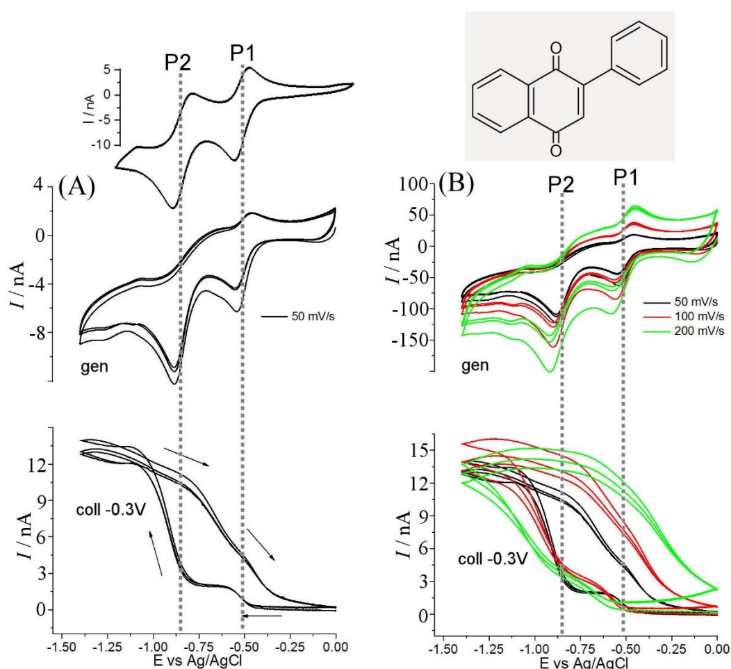
Figure 7. (A) Top: cyclic voltammogram (scan rate 50 mVs -1 ) for the reduction of 5 mM 2-phenylnaphthyl-1,4-dione in dry BMImBF 4 at a 100 μm diameter gold disc electrode. Below: generator-collector gold-gold dual-plate microtrench voltammograms (scan rate 50 mVs -1 , three consecutive cycles, collector potential -0.3 V). (B) As above, but for scan rate 50 mVs -1 (black), 100 mVs -1 (red), and 200 mVs -1 (green).
