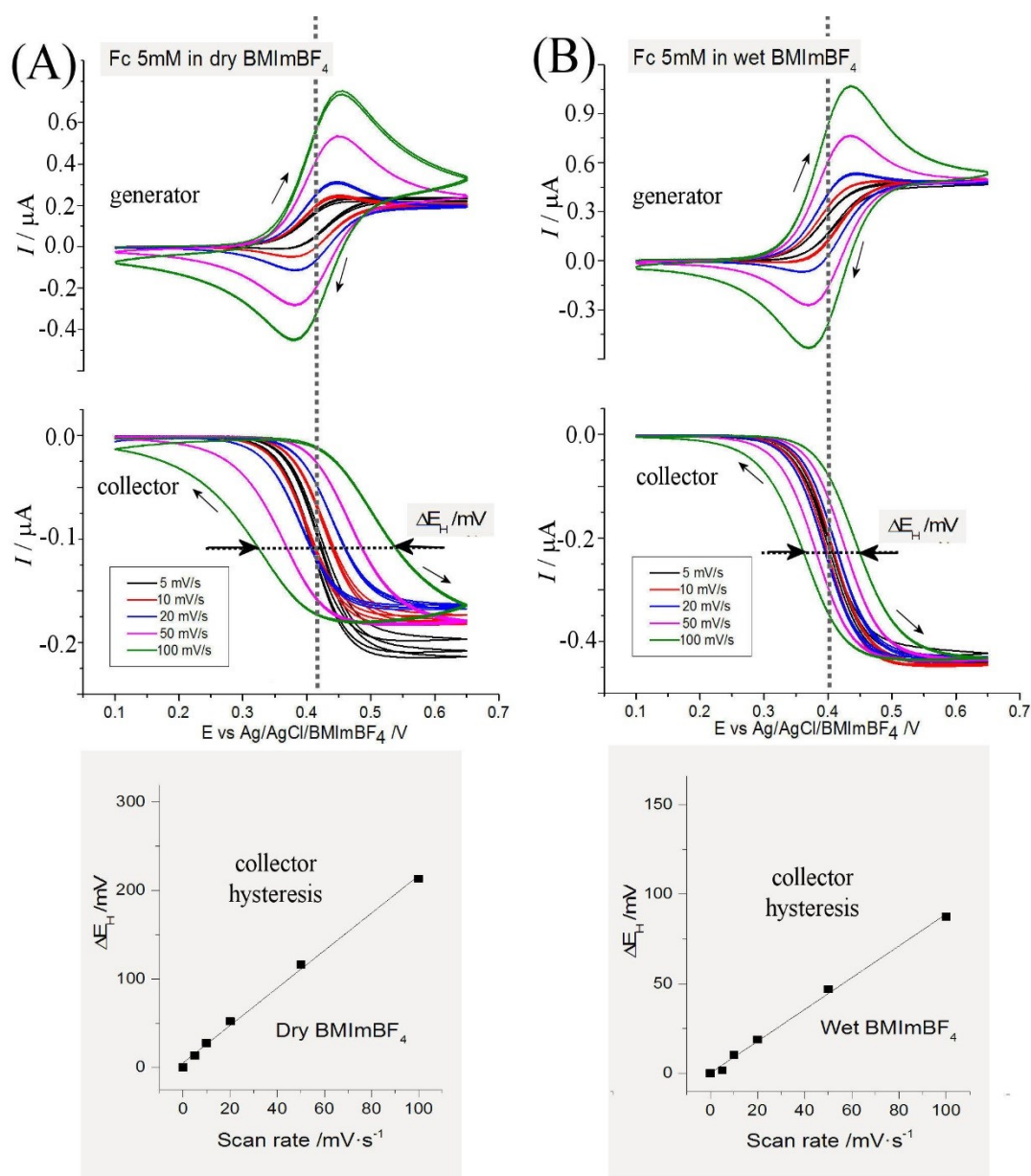
Figure 4. Cyclic voltammograms (Au-Au microtrench, scan rate 5, 10, 20, 50, 100 mVs -1 , collector at 0.1 V) for 5 mM ferrocene in BMImBF 4 (A) under dry conditions (approx. 110 ppm water) and (B) under wet conditions (approx. 5000 ppm water). Linear plots are shown for the collector response hysteresis effect (mV) versus scan rate (mVs -1 ).
