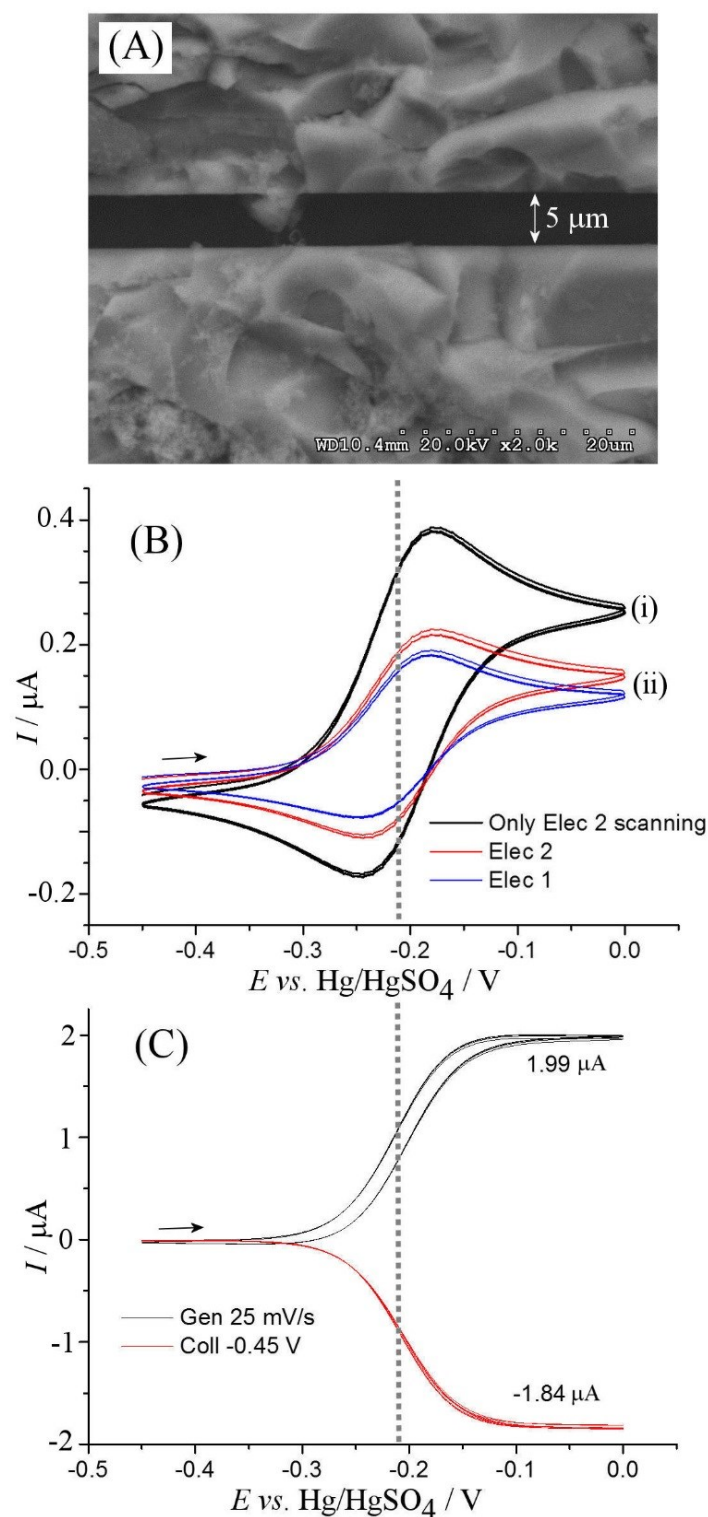
Figure 2. (A) SEM image showing the microtrench with approximately 5 μm inter-electrode gap. (B) Cyclic voltammograms (scan rate 25 mVs -1 ) obtained for oxidation of 1 mM ferrocenemethanol in 0.1 M Na 2 SO 4 for (i) a single electrode connected and (ii) both electrodes independently connected and scanning simultaneously. (C) Cyclic voltammograms (scan rate 25 mVs -1 ; E_{\text{coll}} = -0.45 \text{ V vs. Hg/HgSO}_4 ) in generator-collector feedback mode.
