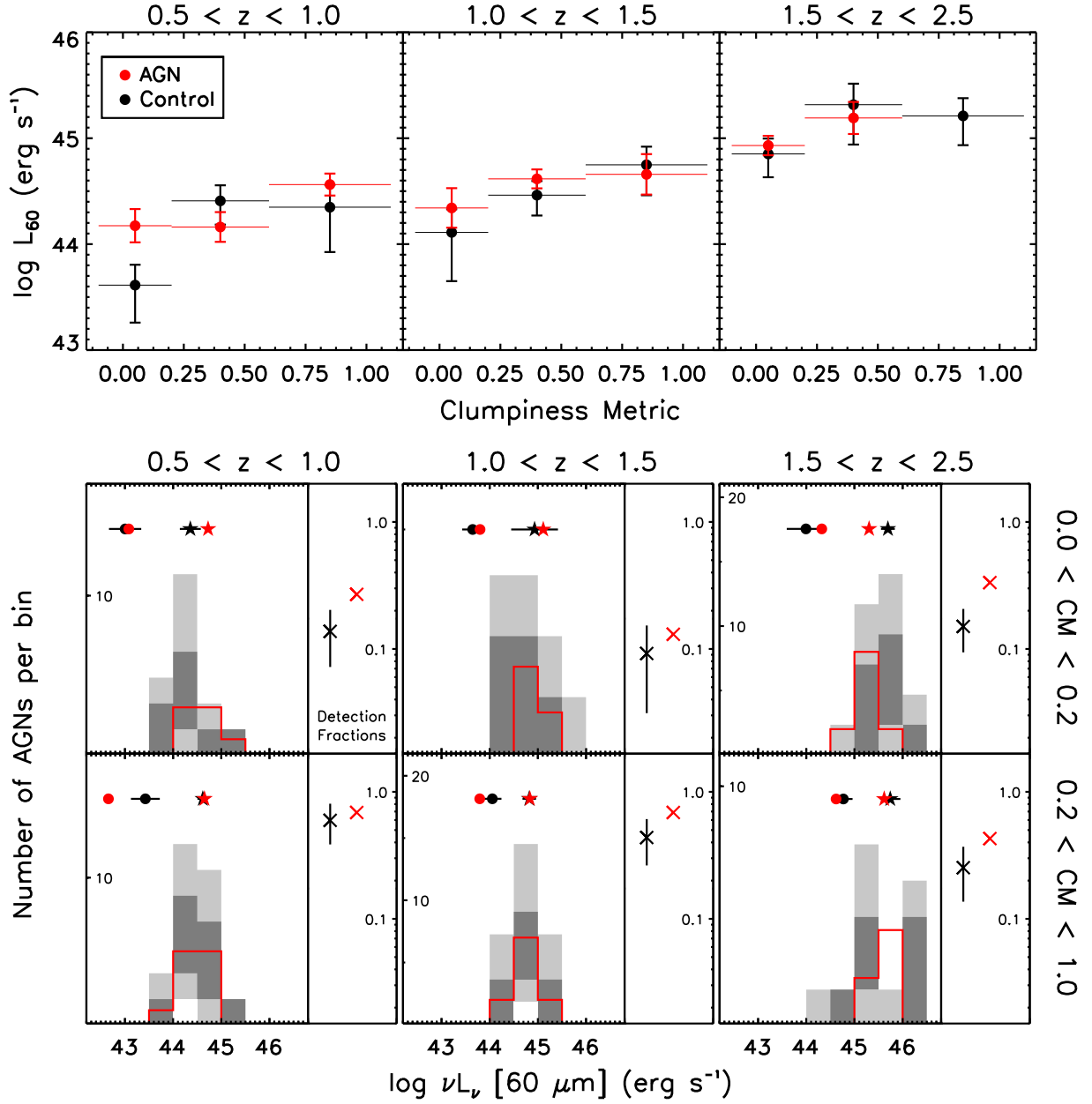
Fig. 15. Mean 60\ \mu\text{m} monochromatic luminosities ( L_{60} ) and luminosity distributions of AGNs and inactive control galaxies in GOODS-S, as a function of visual Clumpiness Metric (CM). Panels left to right span three distinct bins in redshift. In the top row, the mean L_{60} from combinations of detections and stacks are compared in bins of CM. In the lower two rows, each panel is split into two subpanels. L_{60} distributions and PACS detection fractions for AGNs and inactive galaxies are plotted in the left subpanels for two coarse bins in CM. PACS detection fractions are shown in the right subpanels. Details of the plot are identical to those of Figure 13, except for a difference in the structural measure. See Section 4.3 for a discussion.
