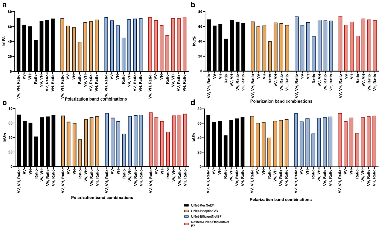
Fig. 14 a–d Show the IoU scores for each model trained with the individual bands VV, VH, (VV + VH)/(VV – VH), and all possible combinations tested on the real datasets from Spain, Kerala, Bihar, and Vietnam, respectively
