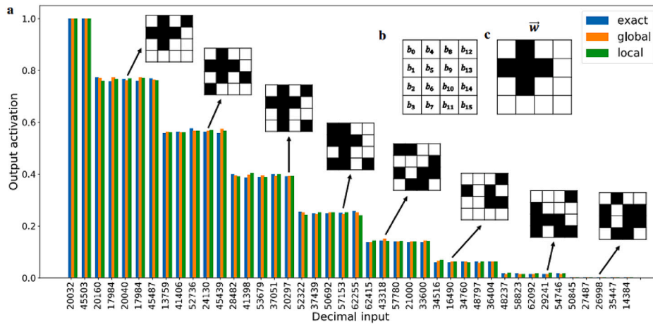
Fig. 29. Classification of 4 \times 4 pixel images [44].
