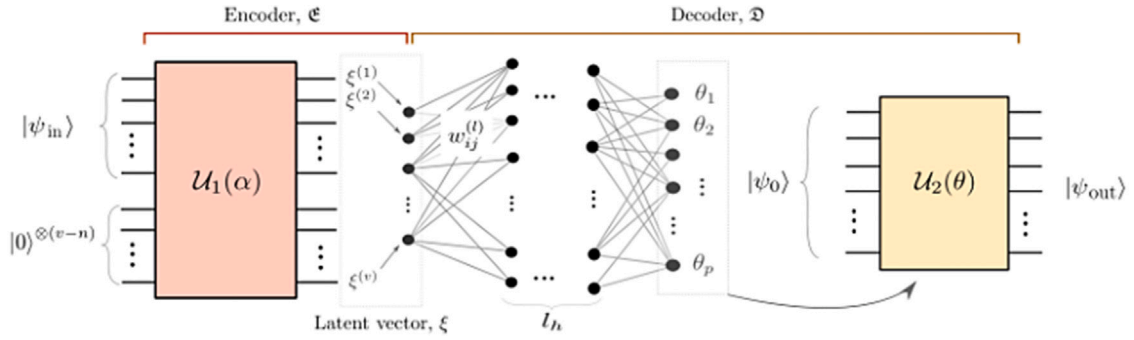
Fig. 5. Hybrid Quantum Autoencoder (HQA) [30].
