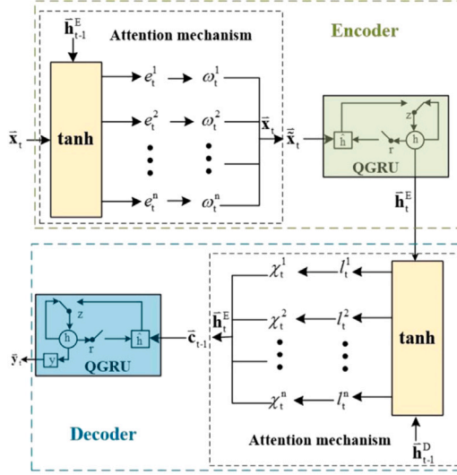
Fig. 26. Quantum recurrent encoding-decoding neural network [56].
