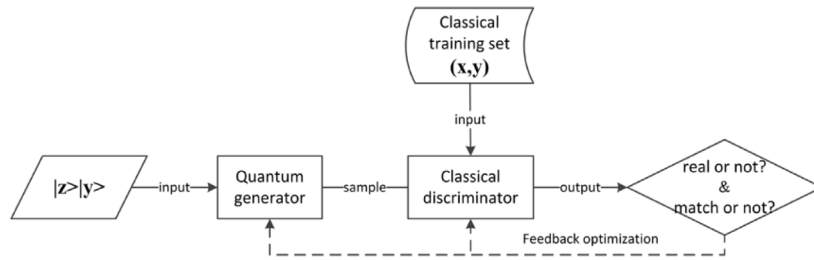
Fig. 23. Conditional adversarial neural networks [48].
