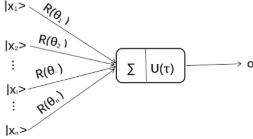
Fig. 9. Quantum neuron model [34].
