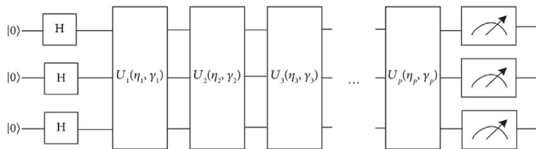
Fig. 22. LSTM-QNN parameterized circuit [45].
