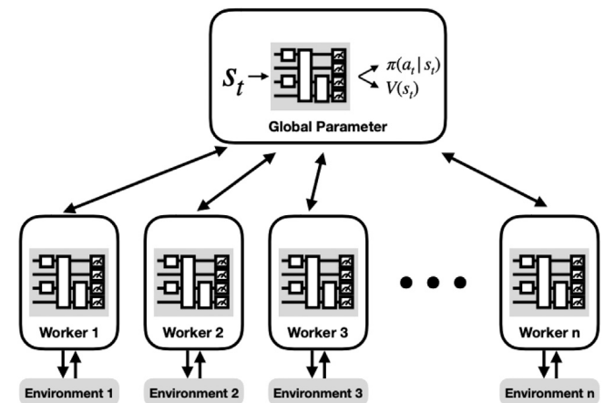
Fig. 4. Quantum asynchronous advantage actor-critic (A3C) learner [52].
