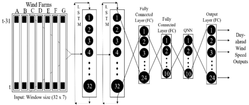
Fig. 21. LSTM architecture [51].
