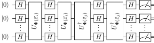
Fig. 8. Quantum circuit of support vector machine [33].
