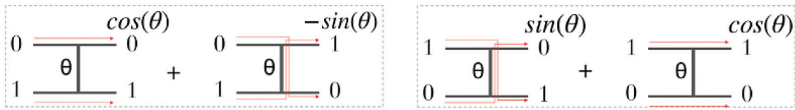
Fig. 12. Quantum mapping in two qubits [40].
