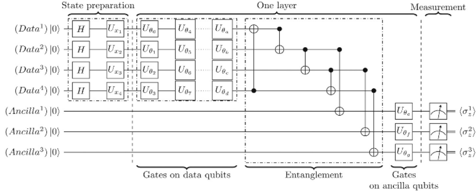
Fig. 6. Quantum variational circuit model [32].
