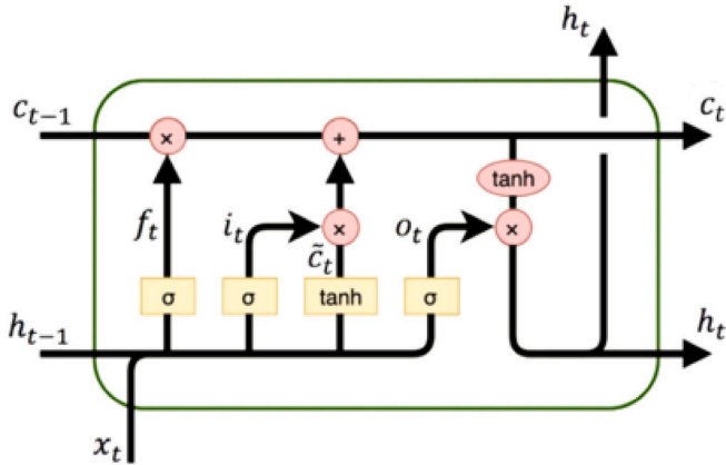
Fig. 20. LSTM cell [50].
