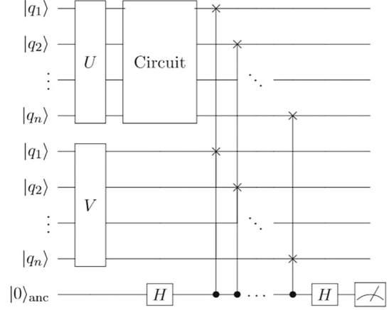
Fig. 11. QKNN circuit [37].
