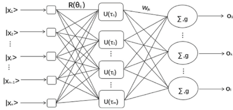
Fig. 18. Quantum backpropagation neural network [34].
