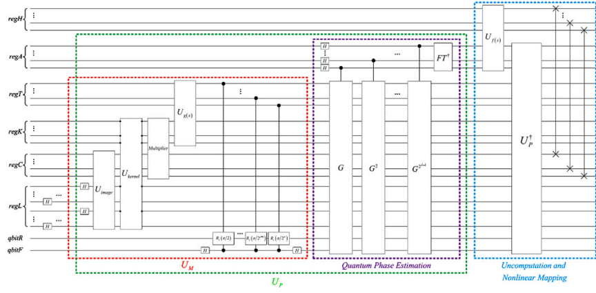
Fig. 16. QDCNN-net architecture [43].
