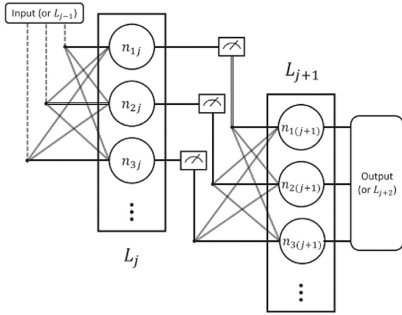
Fig. 19. Feed Forward Neural Network (ffNN) [44].
