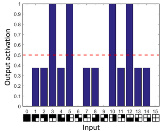
Fig. 28. Classification of 2 \times 2 pixel images [44].
