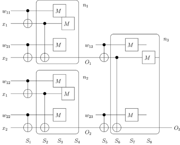
Fig. 15. CNOT quantum neural network [42].
