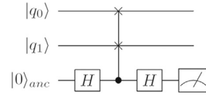
Fig. 10. Test swap circuit [37].
