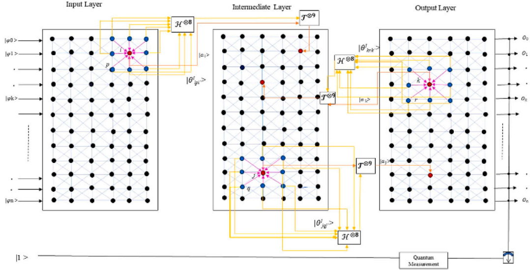
Fig. 14. QFS-Net [41]. (For interpretation of the references to color in this figure legend, the reader is referred to the web version of this article.)
