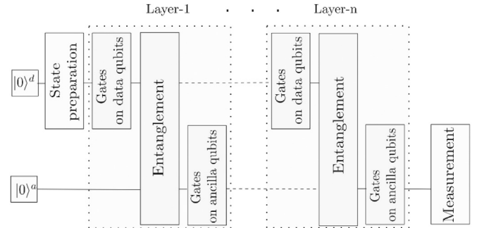
Fig. 7. Architecture of the quantum variational circuit [32].
