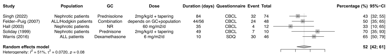
Figure 6. Meta-analysis on the percentage of behavioral changes in glucocorticoid users.
