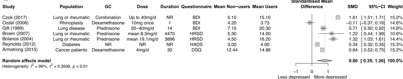
Figure 2. Meta-analysis on the percentage of depression in glucocorticoid users (A). Meta-analysis comparing depression scores between glucocorticoid users and nonusers (B).
