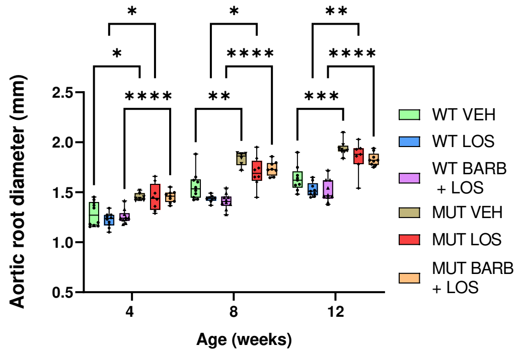
Figure 3. Combined treatment with barbadin and losartan does not show any significant effect on the aortic root diameter of MFS mice compared to losartan alone. Echocardiography data at 12 weeks show that aortic root diameters of MFS mice treated during a period of 8 weeks with barbadin and losartan are not significantly different to those treated with losartan alone. MFS mice from both groups (barbadin and losartan and losartan alone) show a significant dilation compared to the WT controls before the start of the treatment (4 weeks), during the treatment (8 weeks), and after the end of the treatment (12 weeks). A slight decrease in diameter is observed at 8 and 12 weeks for MFS and WT mice of both treated groups compared with the vehicle, but this difference lacks statistical significance. Data are represented as boxplots. Statistical test analysis: One-way ANOVA and Tukey's post-test per timepoint. **** p \leq 0.0001 , *** p \leq 0.001 , ** p \leq 0.01 and * p \leq 0.05 . VEH: vehicle; LOS: losartan; BARB: barbadin; WT: wild type; MUT: mutant.
