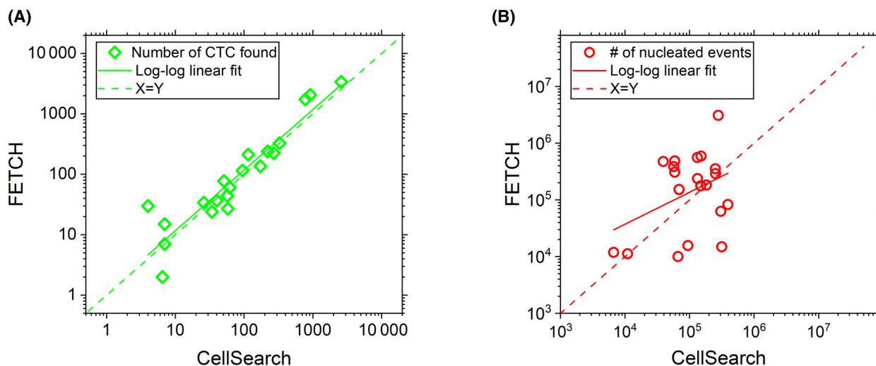
Fig. 4. No CTC loss for FETCH enrichment compared to CellSearch. (A) The number of CTCs and (B) the number of nucleated events obtained from the processing of 20 DLA aliquots each consisting of 2% of the total sample (2%-DLA) using CellSearch or the FETCH showing no loss in CTCs for the FETCH method.
