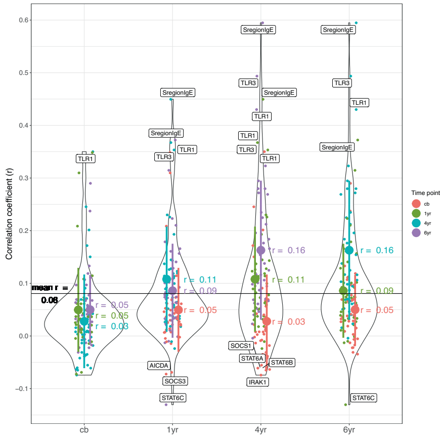
FIGURE 3 Temporal correlation of mRNA expression. Correlations were calculated on 40 genes over 4 time points (6 pairs of time points). The horizontal line shows the overall average (mean) correlation of the mRNA expressions of all pairs of time points. Separate average correlation of genes between each pair of time points is indicated by coloured points and ranges (mean \pm SD). Correlations above r = .35 and below .05 were labelled with gene names. N = 1084 distinct underlying PASTURE individuals involved in calculations (cb, cord blood).
