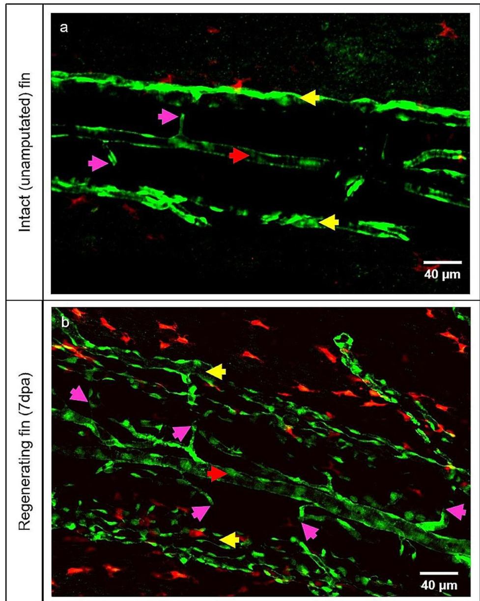
Fig. 3 M \Phi augmentation during the caudal fin regeneration. In vivo appearance of M \Phi by the intact (unamputated) fin ( a ) and regenerating fin at 7dpa ( b ). Blood vessels (ECs) appear in green and M \Phi in red (transgenic line). ( a ) displays hierarchically simple-organized blood vessels containing an artery (red arrow), veins (yellow arrows) and connecting capillaries (purple arrows), and only a few tissue M \Phi . ( b ) displays a dense, complex blood vessel network with multiple M \Phi surrounding the blood vessels and scattered in the tissue in between. Right side – zebrafish tail; images acquired by confocal microscopy
