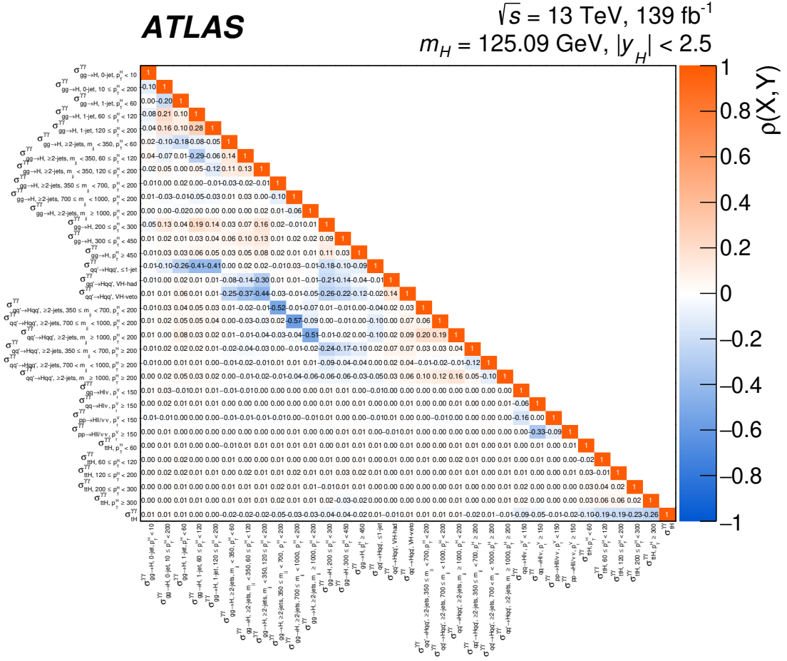
Figure 22. Correlation matrix for the measurement of STXS parameters in each of the 33 regions considered.
