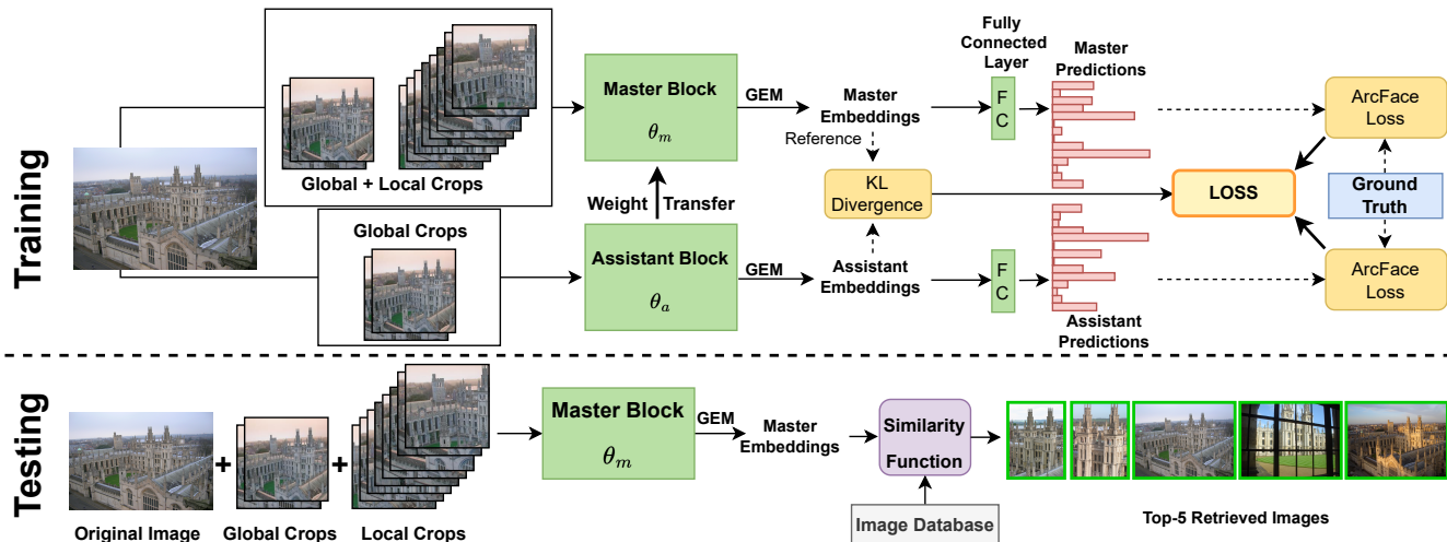
Fig. 1. Training architecture (Upper part): The architecture of the master assistant buddy network (MABNet). Global crops are fed to assistant block while both local and global crops are used for master block to generate assistant and master embedding, respectively, from Generalized Mean Pooling (GEM) layer. KL divergence loss is calculated over these embeddings. The embedding are then passed through a fully connected layer to get predictions, over which ArcFace loss is applied. After each epoch, the weights of master block are updated by weight transfer. Testing architecture (Lower part): The predictions at test time are only performed via the master block. The original input image and its global and local crops are passed to the trained master block to get the embedding from the GEM layer. The concatenation of these embeddings are then compared with the embedding of the images from database with a similarity function (any post-processing method) to retrieve k best images.
