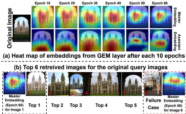
Fig. 2. (a) The superimposed heat map of the the original image after every 10 epochs from both the master and the assistant embedding is generated using Grad-CAM till 60 epochs. (b) Top 5 retrieved image for the original query image. We also show the top 6 retrieved image which is a failure case. The left and right heat map is from the master embedding for the top 1 retrieved image and the failure case, respectively. This result is on Ox105k dataset without post-processing.
