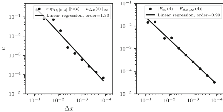
Fig. 5 The errors \sup_{t \in [0,4]} \|u(t) - u_{\Delta x}(t)\|_\infty (left) and |F_\infty(T) - F_{\Delta x,\infty}(T)| at T = 4 (right) plotted against the mesh size \Delta x in Example 5.1
