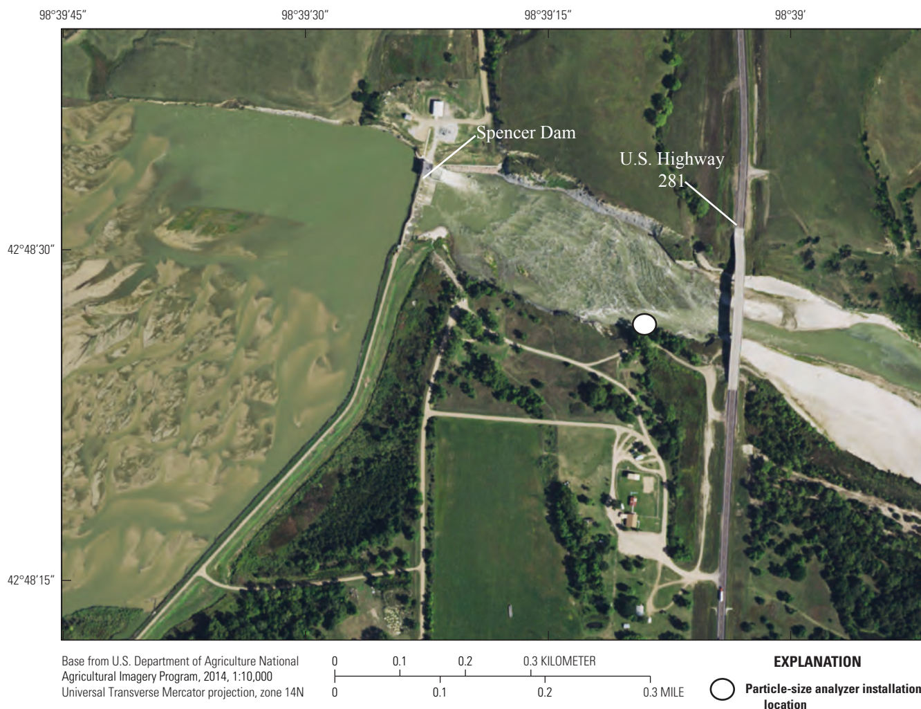
Figure 2. Location of sediment particle-size analyzer at Niobrara River downstream from Spencer Dam, Nebraska, October 2014.
