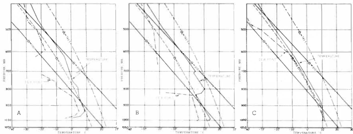
FIGURE 9.—Upper air soundings at Little Rock, Ark. at (A) 0900 est, January 31, (B) 2100 est, January 31, and (C) 0900 est, February 1, 1955.
