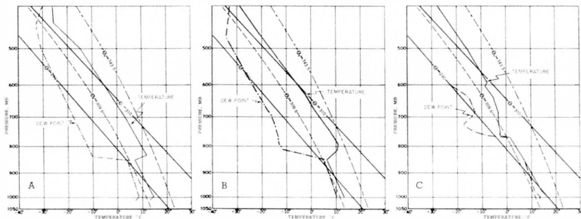
FIGURE 10.—Upper air soundings at Barksdale Air Force Base, Shreveport, La., at (A) 2100 est, January 31, (B) 0300 est, February 1, and (C) 0900 est, February 1, 1955.
