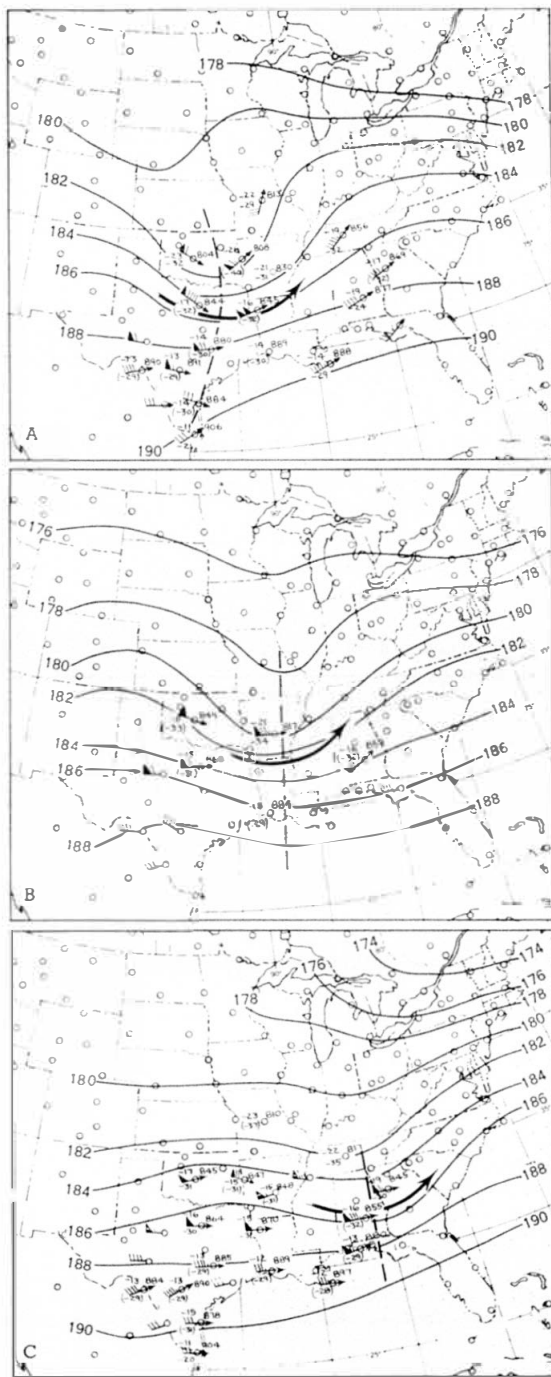
FIGURE 7.—500-mb. charts for February 1, 1955, showing contours (solid lines) for 200-ft. intervals, trough line (dashed) and the current jet position (curved arrow) at (A) 0900 c.s.t., (B) 1500 c.s.t., and (C) 2100 c.s.t.
