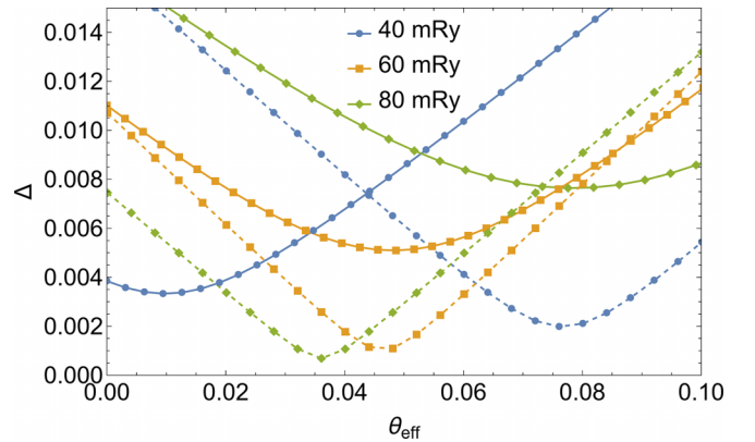
FIG. 10. Fitting error for the spin current \Delta^{(j)} (solid lines) and spin accumulation \Delta^{(\mu)} (dashed lines), as a function of \theta_{eff} at E_F for three different values of disorder. All calculations done at fixed spin-diffusion length as reported in Table I. The fits for the spin current were optimized over the bulk spin Hall conductivity.
