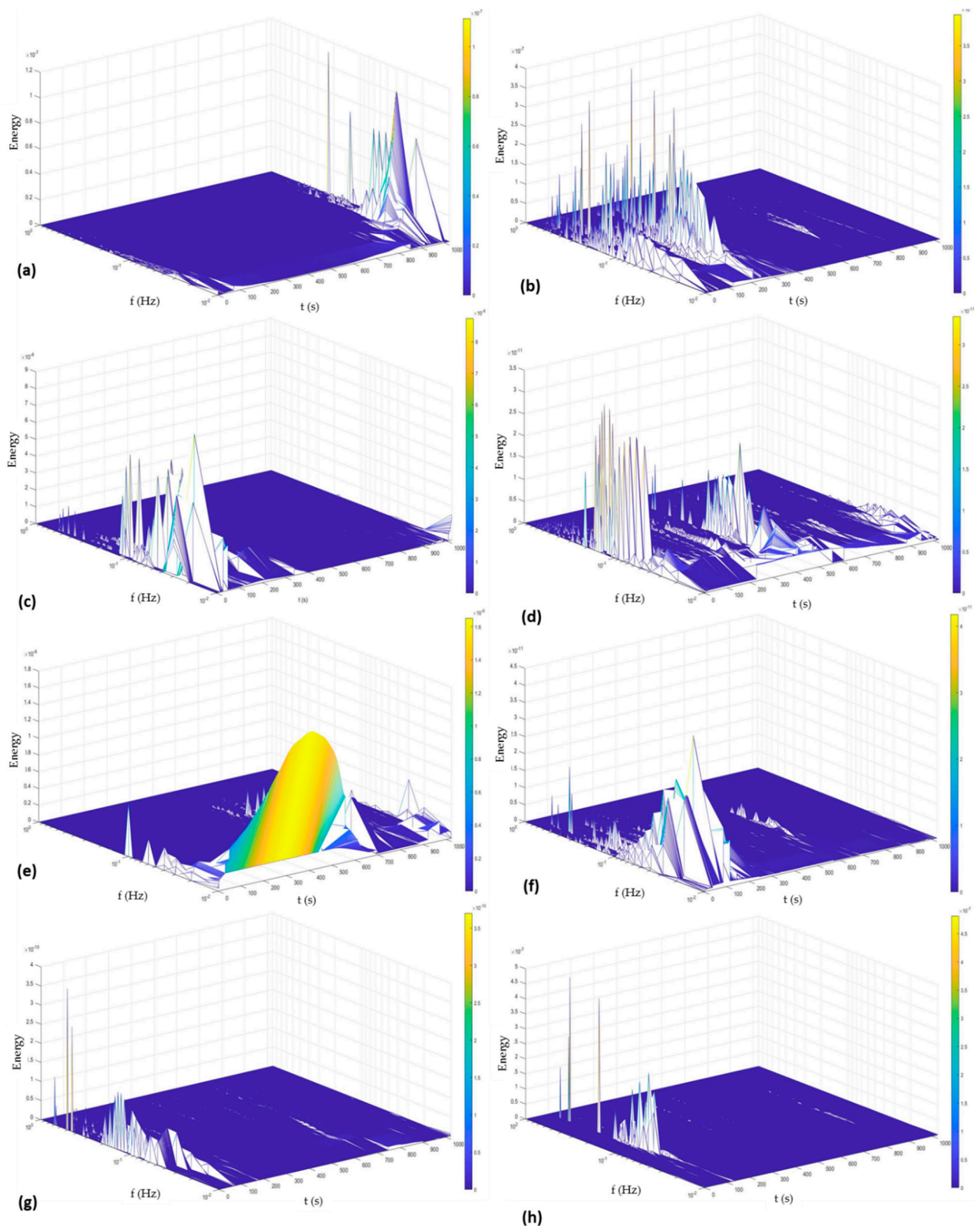
Figure 12. Hilber spectra for AM 350 samples passivated at 49 °C in citric acid (a–d) and nitric acid (e–h) and exposed to NaCl (a,c,e,g) and H 2 SO 4 (b,d,f,h). (a,b,e,f) were passivated 60 min; (c,d,g,h) were passivated 90 min.
