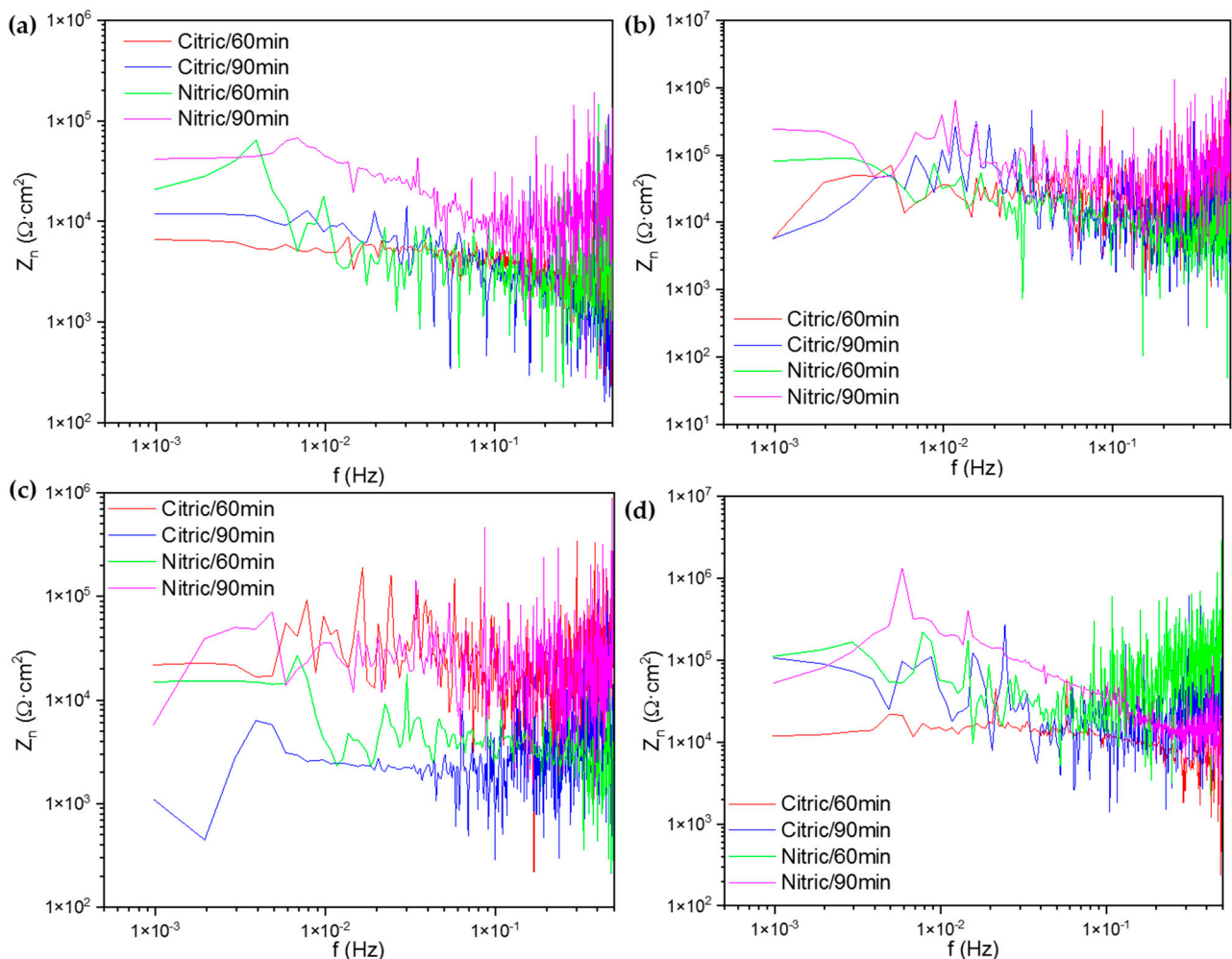
Figure 8. Z_n for AM 350 passivated at 25 °C exposed to (a) NaCl and (b) H_2SO_4 solutions and AM 350 passivated at 49 °C minutes exposed to (c) NaCl and (d) H_2SO_4 solutions.
