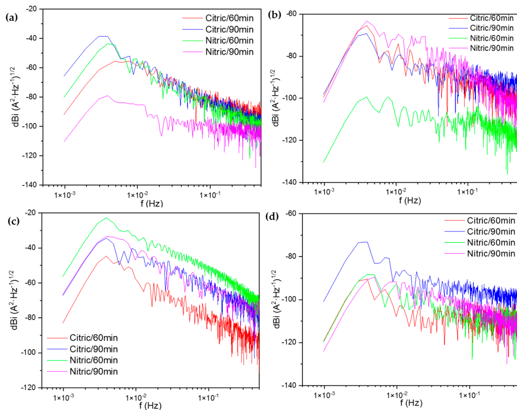
Figure 5. PSDs in currents for Custom 450 passivated at 25 °C exposed to (a) NaCl and (b) \text{H}_2\text{SO}_4 solutions and Custom 450 passivated at 49 °C exposed to (c) NaCl and (d) \text{H}_2\text{SO}_4 solutions.
