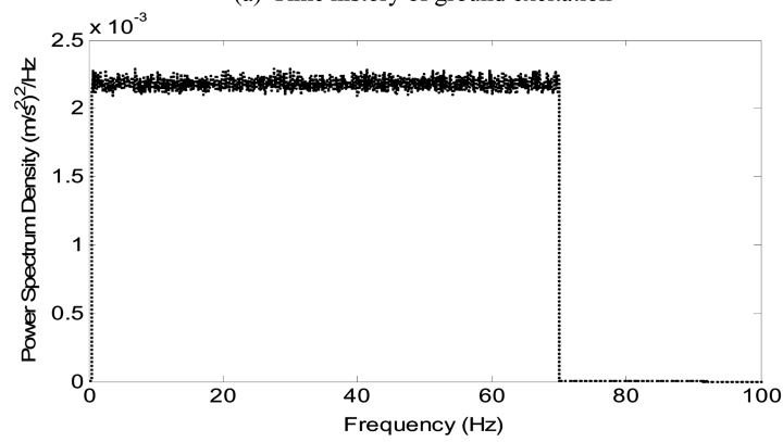
(b) Power spectrum density of ground excitation
