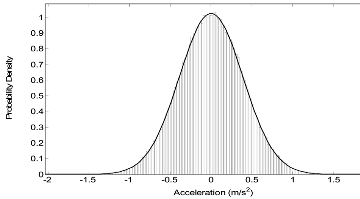
(c) Probability density distribution of ground excitation
