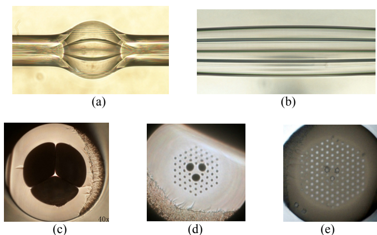
Fig. 1. Side-view of microcells produced by (a) arc discharge and (b) flame brushing. Cross-section of a microcell at different locations along the cell: (c) at the center, (d) at the transition region, and (e) away from the cell.
