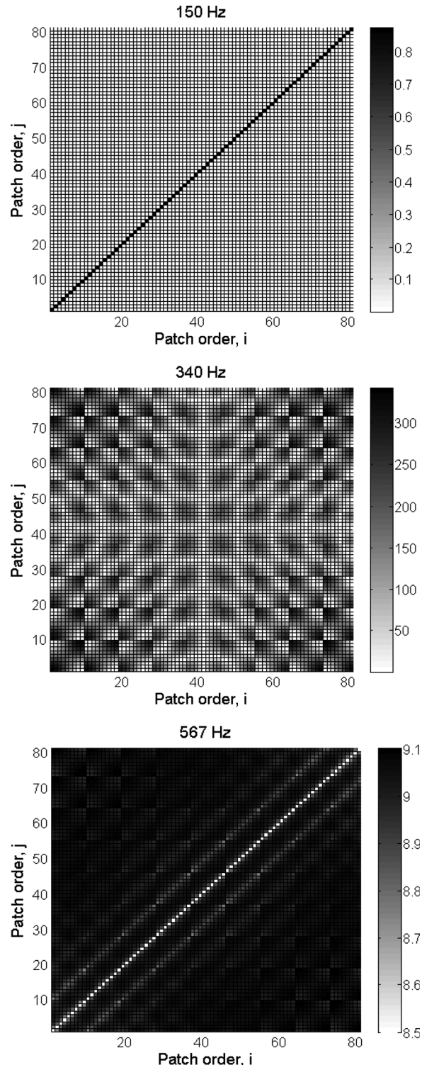
FIG. 6. Magnitude of the equivalent patch transfer functions [N/(m/s)].
