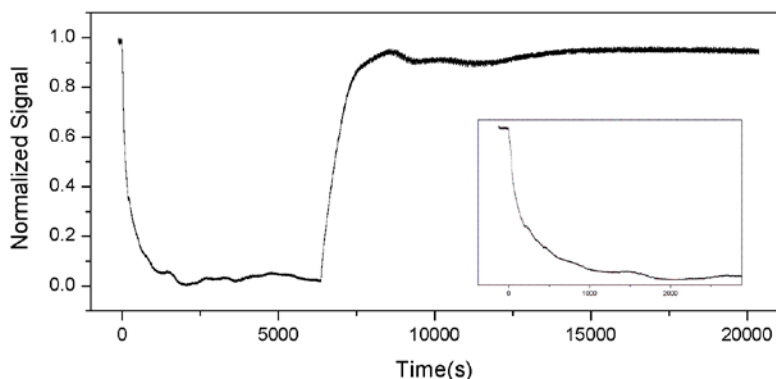
Fig. 2. Output signal measured from a 3-m long HC-1550-02 fiber with 12 micro-channels evenly distributed along the fiber. The gas acetylene concentration used is \sim 1\% .
