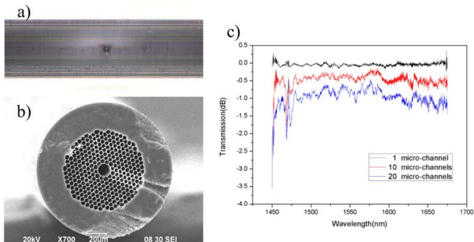
Fig. 1. (a) Side-view and (b) cross-section of a micro-channel fabricated on the HC-1550-02 fiber. (c) Loss spectrum of a 30 cm long HC-1550-02 fiber with 10 and 20 micro-channels evenly distributed along the fiber.
