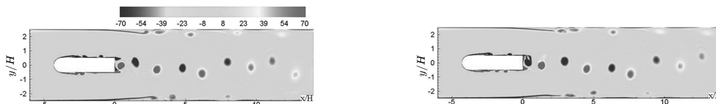
Figure 6: Vorticity distributions within a half cycle of lift variation for D/H = 2
