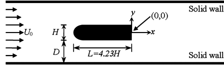
Figure 1: Schematic sketch of the problem
