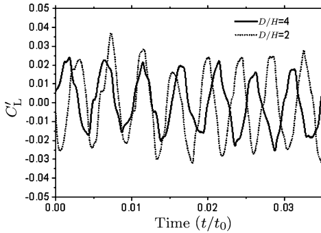
Figure 2: Time evolution of C'_L for different gap ratios
