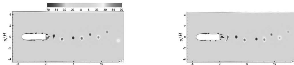
Figure 5: Vorticity distributions within a half cycle of lift variation for D/H = 4
