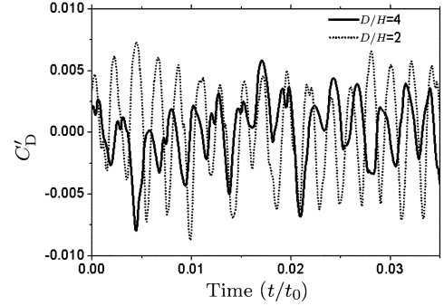
Figure 3: Time evolution of C'_D for different gap ratios
