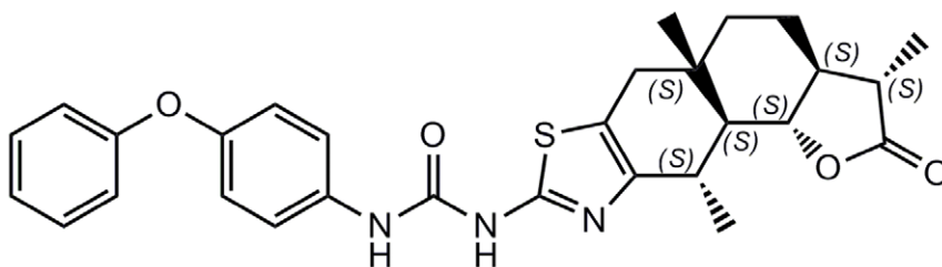
Figure 1. Chemical structure of carbamide 1. doi:10.1371/journal.pone.0043278.g001
