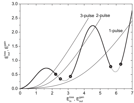
Fig. 12. Periodic nonlinear loss and saturating gain curves for one-pulse, two-pulse, and three-pulse per round trip configurations. The intersection of the gain and loss curves represents the mode-locked solution states of interest. As the cavity energy is increased, the gain curves shift to the right. The one-pulse solution first experiences periodic and chaotic behavior before ceasing to exist beyond the threshold point indicated by the rightmost bold circle. The solution then jumps to the next most energetically favorable configuration of two pulses per round trip. However, a high-energy one-pulse solution can also exist.
