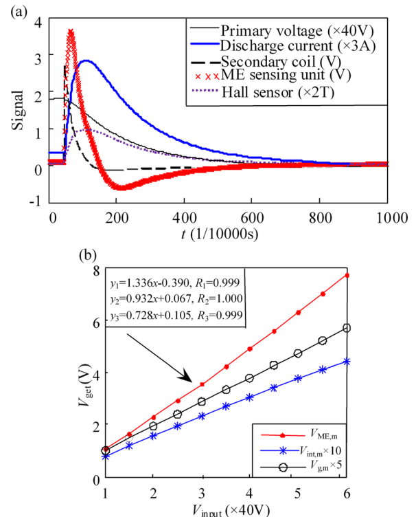
FIG. 2. (Color online) Calibration of ME sensing unit: (a) typical acquired waveforms for conducting magnetic measurements; (b) the measured maximum values of V_{\text{ME}} , V_{\text{int}} , V_g as a function of V_{\text{input}} .
