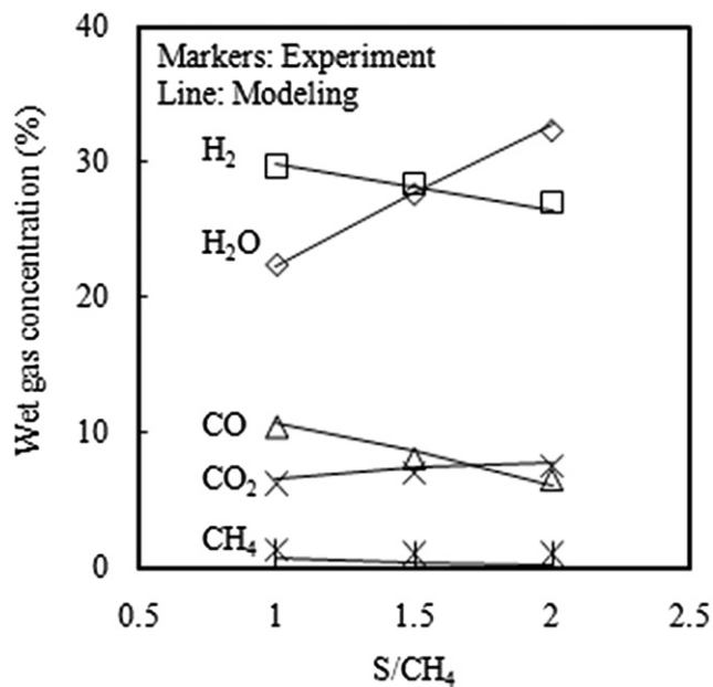
Fig. 3 – Comparison between predicted and measured [26] gas concentrations at different S/\text{CH}_4 ratios in an ATR reformer.
