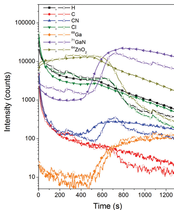
FIG. 5. (Color online) SIMS profiles for DN (closed symbols) and DA (open symbols) samples.
